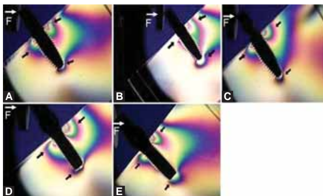
Figs 3A to E: (A) Implant-abutment of EH with load II (Alvim Ti), (B) implant-abutment of IH-PS with load II (Alvim II Plus), (C) implant-abutment of MC with load II (Alvim CM), (D) implant-abutment of IH with load II (Full Osseotite), (E) implant-abutment of IH-PS with load II (Certain Prevail)
