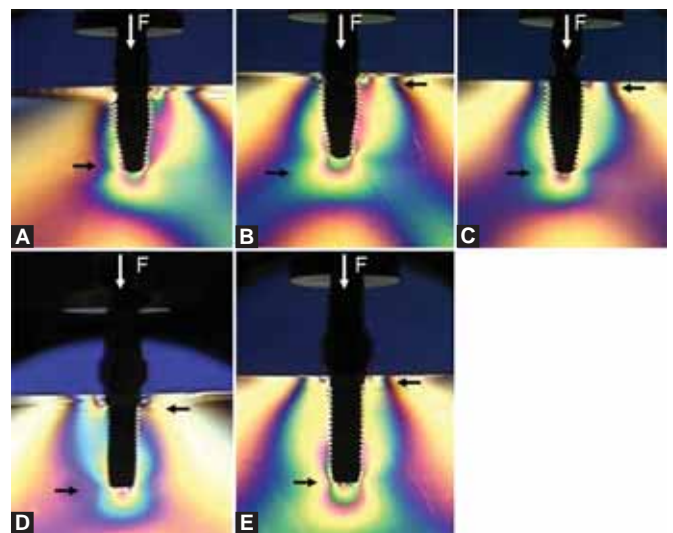
Figs 2A to E: (A) Implant-abutment of EH with load I (Alvim Ti), (B) implant-abutment of IH-PS with load I (Alvim II Plus), (C) implant-abutment of MC with load I (Alvim CM), (D) implant-abutment of IH with load I (Full Osseotite), (E) implant-abutment of IH-PS with load I (Certain Prevail)
