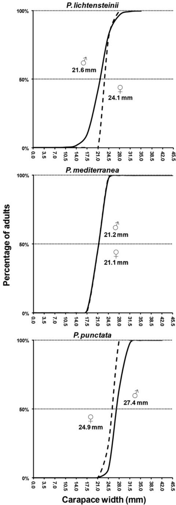
Fig. 3. Size at the onset of morphological sexual maturity for each Persephona species and sex (— = males; --- = females).
