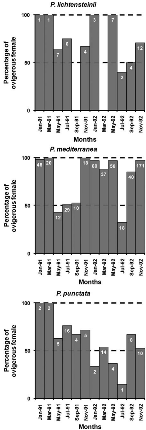
Fig. 4. Variation in the percentage of ovigerous females in relation to mature females sampled in the population during the study period, for Persephona lichtensteinii , Persephona mediterranea , and Persephona punctata (numbers above each bar correspond to the total individuals collected).
