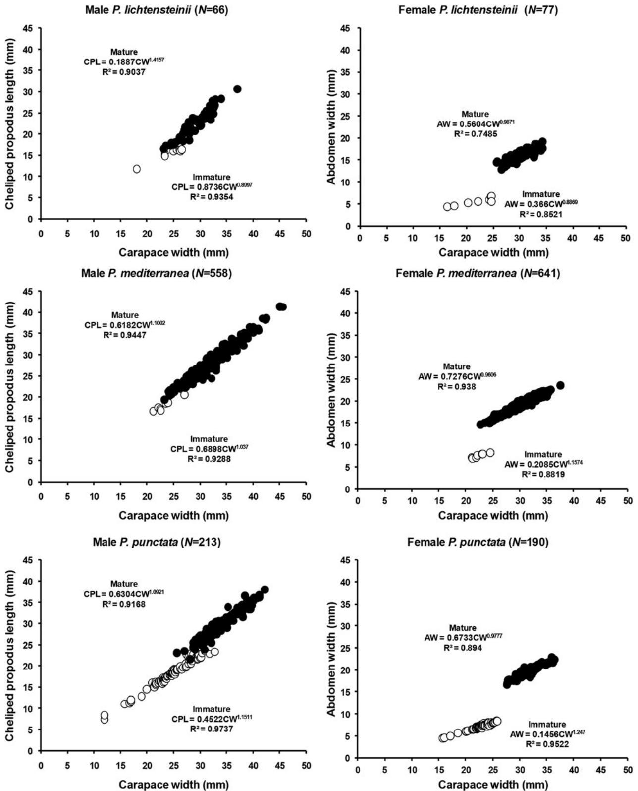
Fig. 2. Morphometric relationships between carapace width (CW), cheliped propodus length (CPL), and abdomen width (AW) for males and females of Persephona lichtensteinii , Persephona mediterranea and Persephona punctata .
