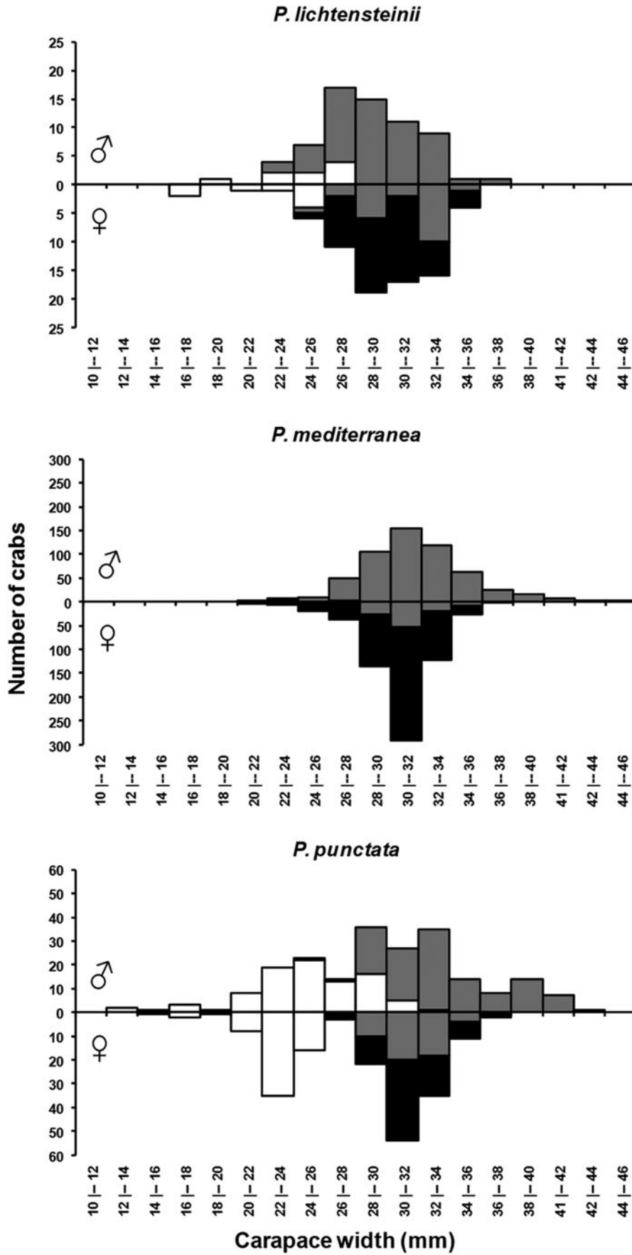
Fig. 1. Size–frequency distributions for all species and both sexes (white bar = juvenile males and females; grey bar = adult males and females; black bar = ovigerous females).
