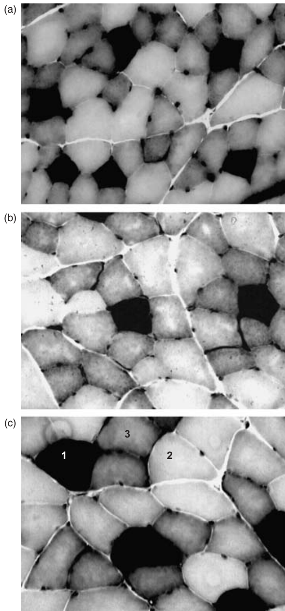
Figure 1 Flexor carpi radialis muscle (40 \times ) of crossbred female rabbits slaughtered at 42 (a), 63 (b) and 84 days of age (c). Notice the three types of fibers: I (1), IIA (2) and IIB/X (3) and also the hypertrophy in the more advanced age. ATPase, after acid pre-incubation (pH = 4.5).
