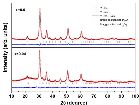
Fig. 2. XRD patterns after structural refinement procedure using Rietveld method for the \text{In}_{2-x}\text{Er}_x\text{O}_3 nanostructures, x= mol of \text{Er}^{3+} ions.
