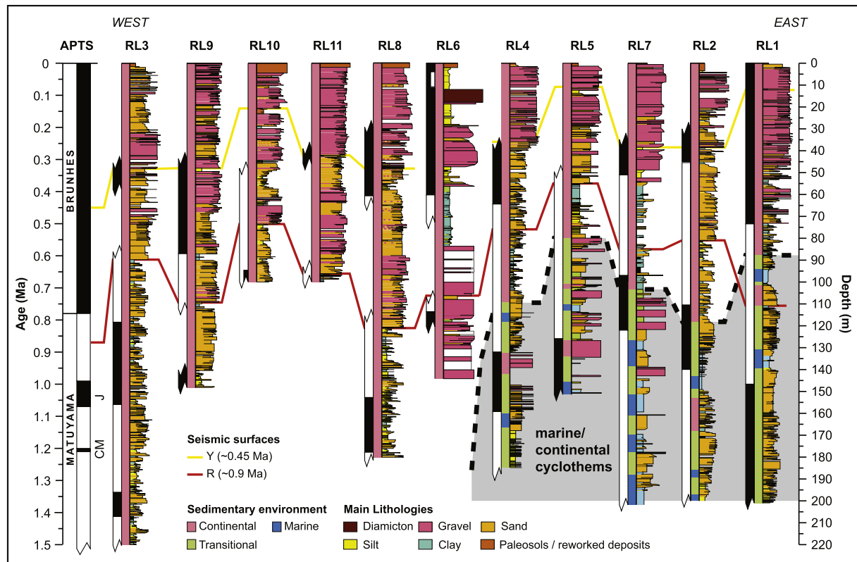
Fig. 9. Po Plain cores, ordered longitudinally from west (Cilavegna RL3) to east (Ghedì RL1) (see Fig. 3 for geographic locations), correlated by means of magnetostratigraphy to the astrochronological polarity time scale (APTS; Lourens et al., 2005). The 'R' surface and 'Y surface' are also indicated by red and yellow correlation lines, respectively. The lateral eastward transition from full continental to marine/continental cyclothem (dashed line) is also shown based on the lithostratigraphy of the cores. J = Jaramillo, CM = Cobb Mountain. See text and Scardia et al. (2012) for additional information.
