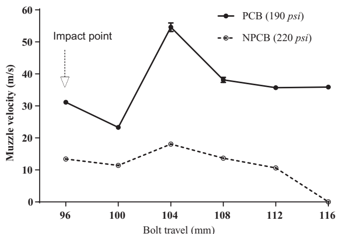
Fig. 2. Profiles of muzzle velocity for penetrative captive bolt (PCB) and non-penetrative captive bolt (NPCB) guns.
