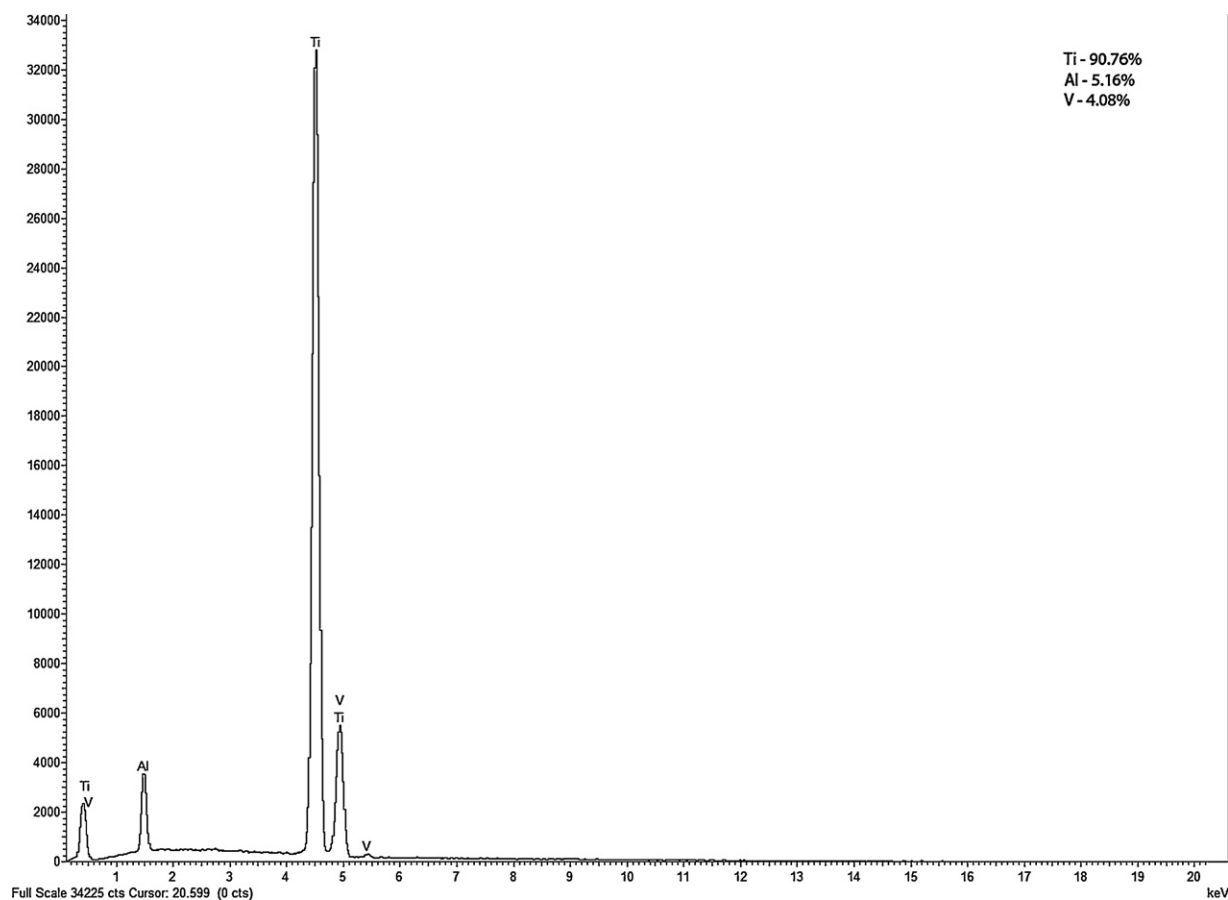
Fig. 8 – Semi-quantitative composition of Ti-6Al-4V after brushing with fluoride toothpaste (Group BFT).
