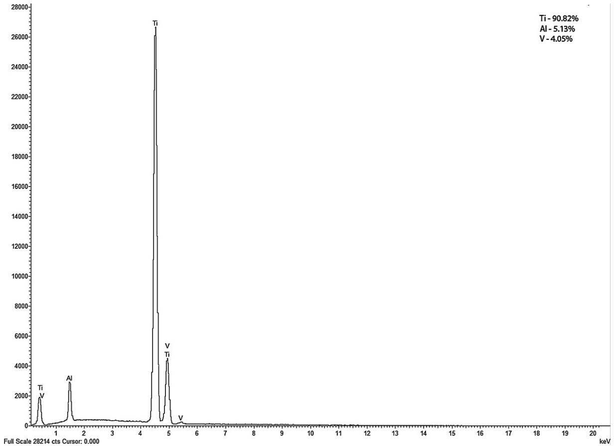
Fig. 7 – Semi-quantitative composition of Ti-6Al-4V after immersion in fluoride toothpaste (Group IFT).
