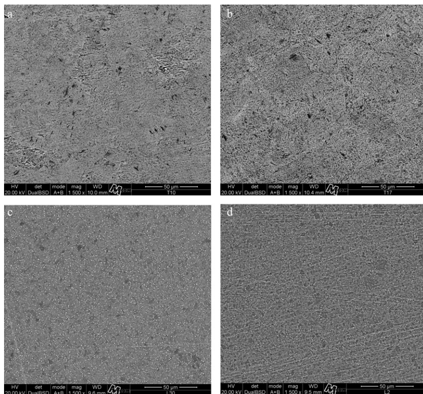
Fig. 4 – Scanning electron microscope images (1500×) of samples exposed to fluoride ions; cp Ti – Group IFT (a), Group BFT (b); Ti-6Al-4V – Group IFT (c) and Group BFT (d).
