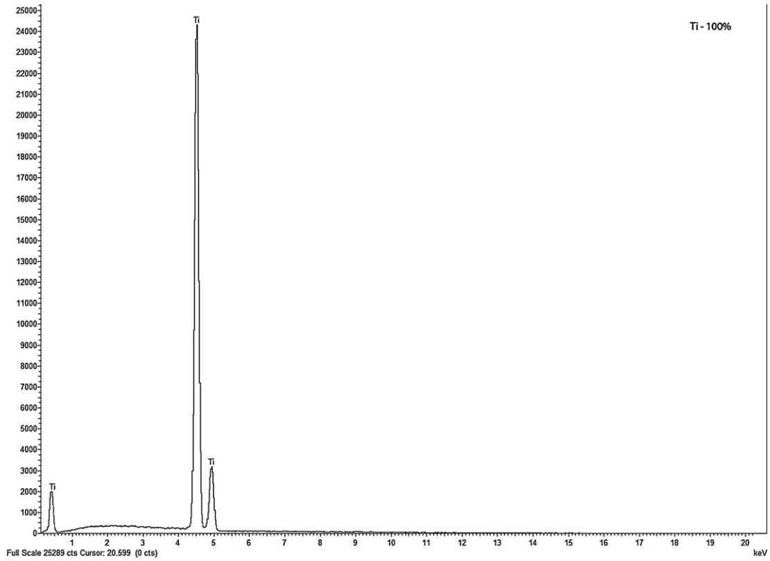
Fig. 6 – Semi-quantitative composition of cp Ti after brushing with fluoride toothpaste (Group BFT).
