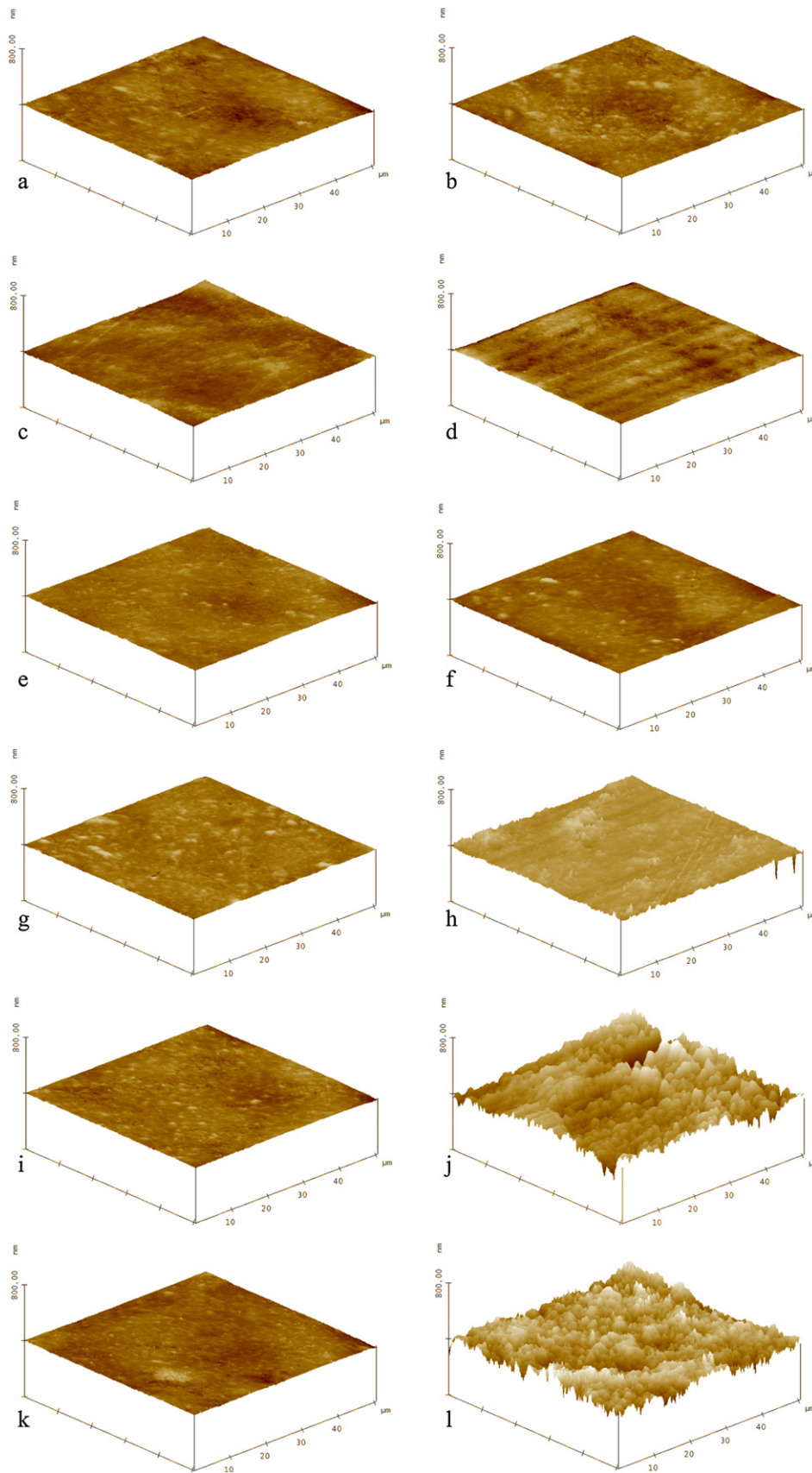
Fig. 2 – 3D atomic force microscopy images of cp Ti. Group IW pretreatment (a) and post-treatment (b); Group IT pretreatment (c) and post-treatment (d); Group IFT pretreatment (e) and post-treatment (f); Group BW pretreatment (g) and post-treatment (h); Group BT pretreatment (i) and post-treatment (j); Group BFT pretreatment (k) and post-treatment (l). The colour becomes lighter on proceeding from the valleys towards the peaks.
