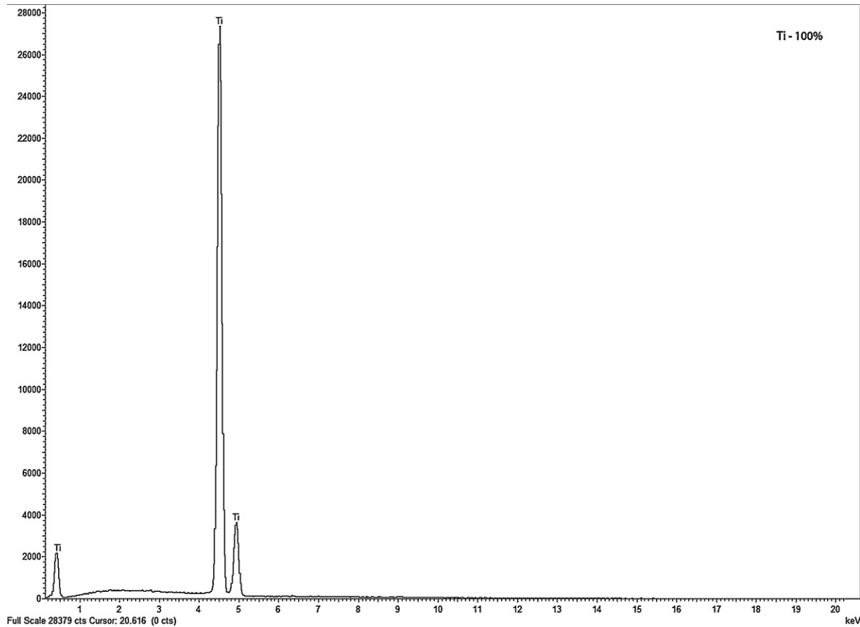
Fig. 5 – Semi-quantitative composition of cp Ti after immersion in fluoride toothpaste (Group IFT).
