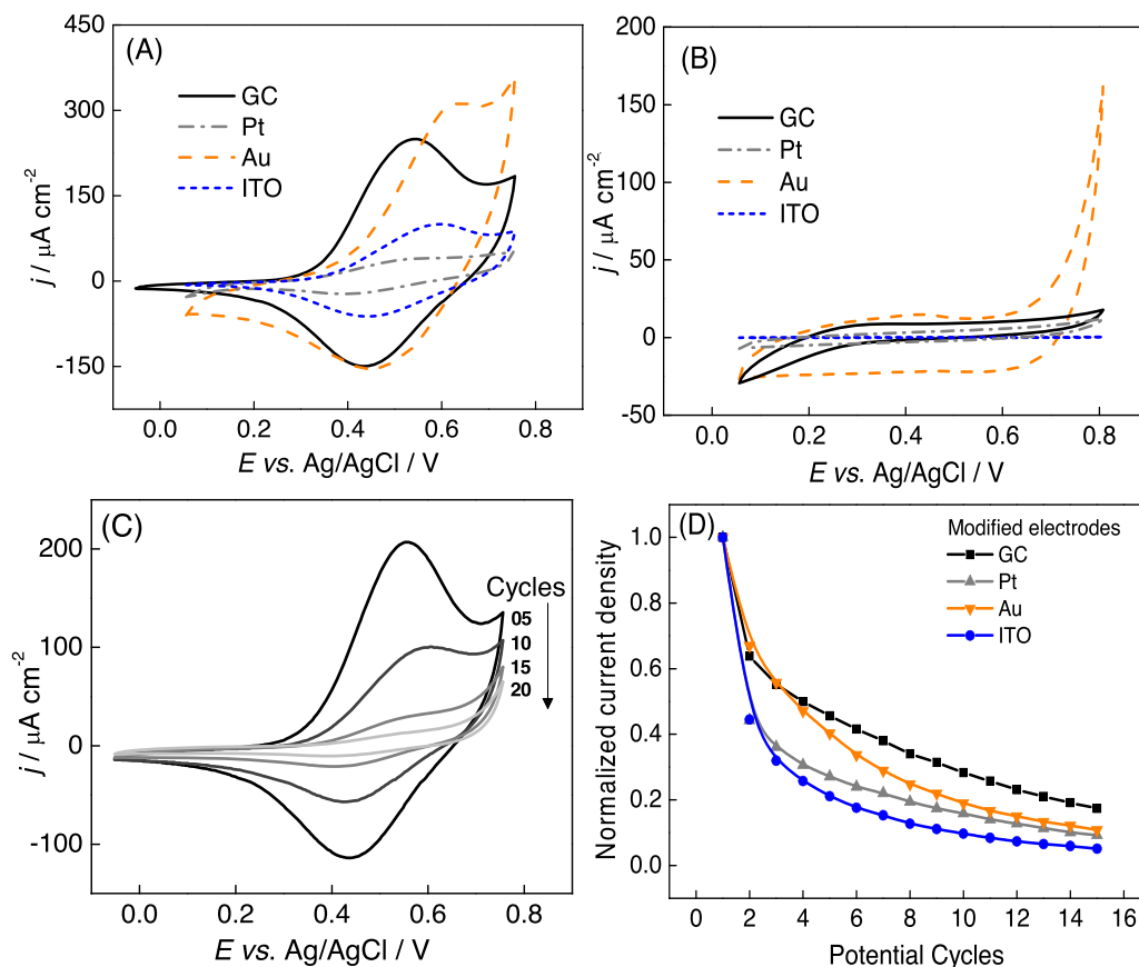
Fig. 2. Cyclic voltammetry in 0.1 mol L -1 KCl aqueous solution; \nu = 25 mV s -1 ; third cycle, for GC, Pt, Au and ITO electrodes (A) modified with Ni-Salpn and (B) unmodified. (C) Voltammetric response during cycle 5, 10, 15 and 20 for GC electrode substrate (D) Variation of current density with number of potential cycles for modified GC, Pt, Au and ITO electrode substrates.
