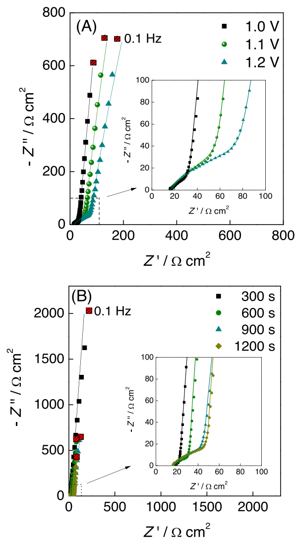
Fig. 4. Complex plane impedance spectra of GC electrodes modified with Ni-Salpn films in 0.1 mol L -1 KCl solution at OCP (+0.36 V vs. Ag/AgCl). Magnifications of the high frequency part are also shown. Lines indicate equivalent circuit fitting. (A) For different electrodeposition potentials (+1.0 V, +1.1 V, +1.2 V vs. Ag/AgCl for 900 s), (B) For different electrodeposition times (300 s, 600 s and 900 s at +1.2 V vs. Ag/AgCl).
