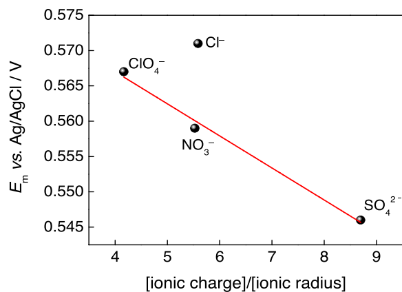
Fig. 10. Dependence of the mid-potential, E_m , of the GC electrode modified with Ni-Salpn thin film vs. [\text{ionic charge}]/[\text{ionic radius}] of counteranions. The values of ionic radius in aqueous solutions were from [48].
