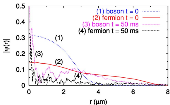
FIG. 2. (Color online) The initial ( t=0 ) and final ( t=50 ms) fermion and boson wave functions in arbitrary units before and after collapse initiated by a jump in boson-fermion scattering length a_{BF} from -12.5 to -37.5 nm.
