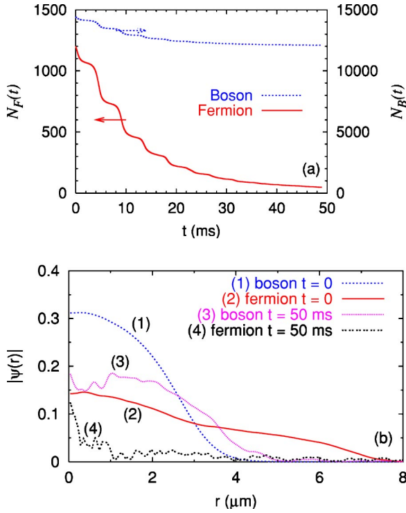
FIG. 4. (Color online) (a) The evolution of the numbers of bosons N_B(t) and fermions N_F(t) during collapse initiated by a jump in the boson number from 4800 to 14 400 for K_3=10^{-27} \text{ cm}^6 \text{ s}^{-1} . (b) The initial ( t=0 ) and final ( t=50 ms) fermion and boson wave functions in arbitrary units before and after the collapse in (a).
