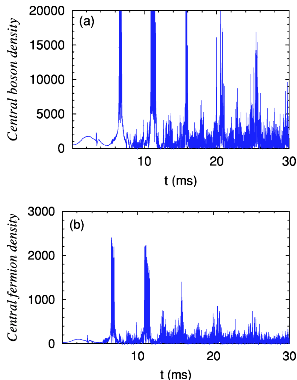
FIG. 3. Evolution of the (a) central boson probability density [N_B|\psi_B(0,t)|^2] and (b) central fermion probability density [N_F|\psi_F(0,t)|^2] in arbitrary units during the collapse exhibited in Figs. 1 and 2.
