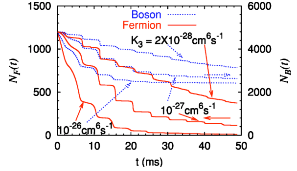
FIG. 1. (Color online) The evolution of the numbers of bosons N_B(t) and fermions N_F(t) during collapse initiated by a jump in boson-fermion scattering length a_{BF} from -12.5 to -37.5 nm for K_3=2 \times 10^{-28} , 10^{-27} , and 10^{-26} \text{cm}^6 \text{s}^{-1} . The three upper (blue, dotted) curves refer to number of bosons and three lower (red, solid) curves refer to number of fermions. The curves are labeled by their respective K_3 values.
