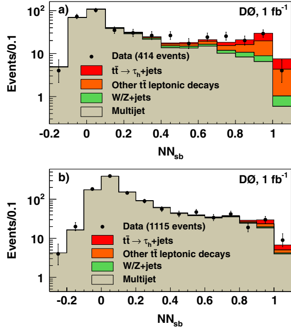
FIG. 1 (color online). The output of NN_{sb} for (a) the tau-type 1 and 2 channel, (b) the tau-type 3 channel. The \chi^2 per degree of freedom between data and templates is 0.6 for (a) and 0.5 for (b).
