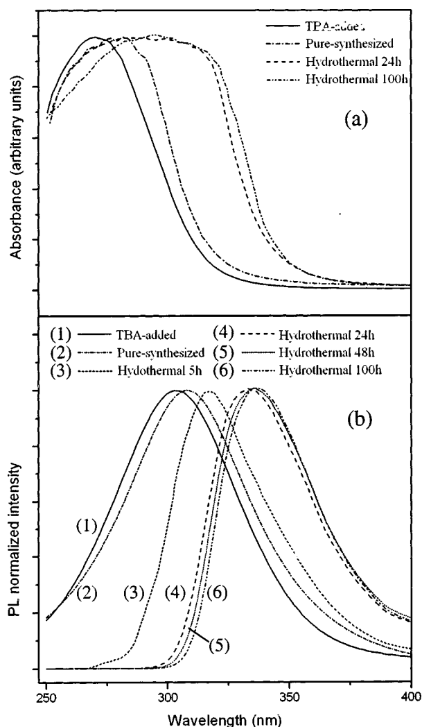
FIG. 2. Optical characterization of the \text{SnO}_2 colloidal suspensions: (a) Absorbance spectra measured by UV-vis of nanoparticles of different size and (b) photoluminescence emission spectra of excitation of \lambda = 250 nm. All measurements were carried out at room temperature.
