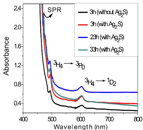
FIG. 2. (Color online) Absorbance spectra of the GGSPr sample (with and without metallic nanoparticles) for different annealing times as indicated in the legend. Sample thickness: 3.9 nm.
