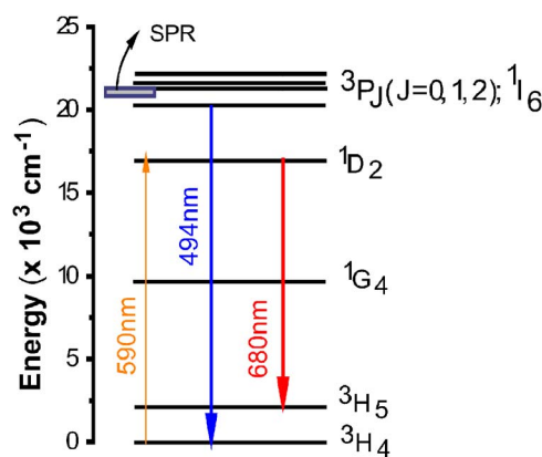
FIG. 4. (Color online) Simplified energy level diagram for \text{Pr}^{3+} ions.
