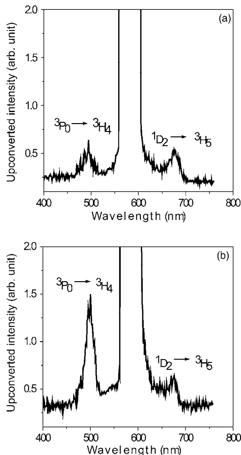
FIG. 3. Luminescence spectra for the samples heat treated during 23 h (excitation wavelength: 590 nm): (a) GGSPr and (b) GGSAgPr. The strong signal centered at 590 nm is due to the scattered laser beam.
