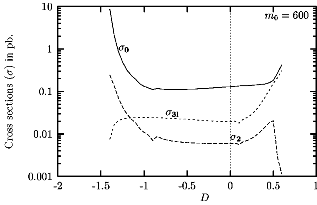
FIG. 1. Cross sections (in pb, without any cut) for different final states at the Tevatron collider with \sqrt{s}=2 TeV as a function of D . The other relevant parameters are m_{1/2}=105 GeV, m_0=600 GeV and \tan\beta=3 , while \mu is fixed by imposing the radiative electroweak symmetry breaking condition for D=0 .
