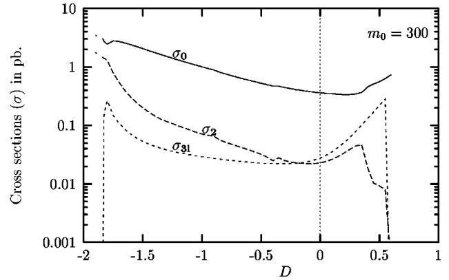
FIG. 2. As in Fig. 1, but with m_0=300 GeV.
