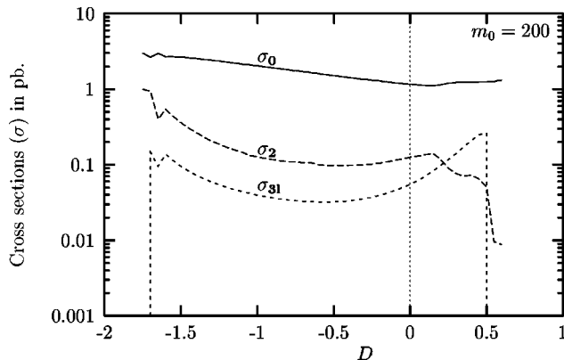
FIG. 3. As in Fig. 1, but with m_0=200 GeV.
