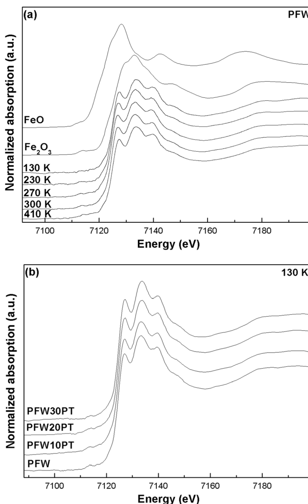
FIG. 1. XANES spectra at Fe K-edge for (a) PFW sample and Fe oxides standards as a function of temperature and (b) PFW-PT samples as a function of \text{PbTiO}_3 content.
