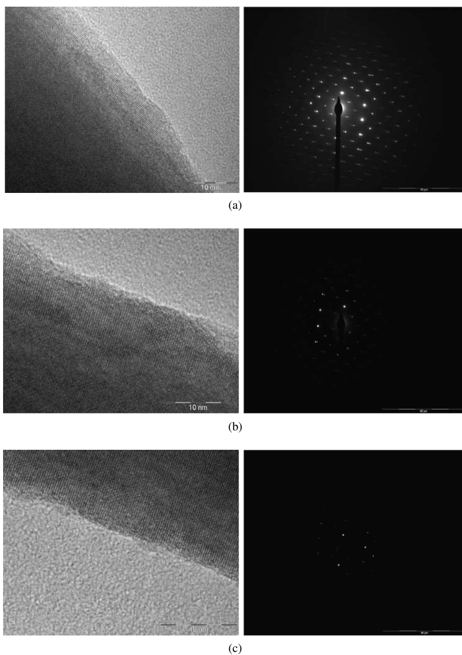
Figure 6. TEM and SAD images of Y_3Fe_{5-x}Al_xO_{12} powders synthesized at 700\text{ }^\circ\text{C} for 2 h by the polymeric precursor method with: a) x = 1.5 , b) x = 1.6 and c) x = 1.7
