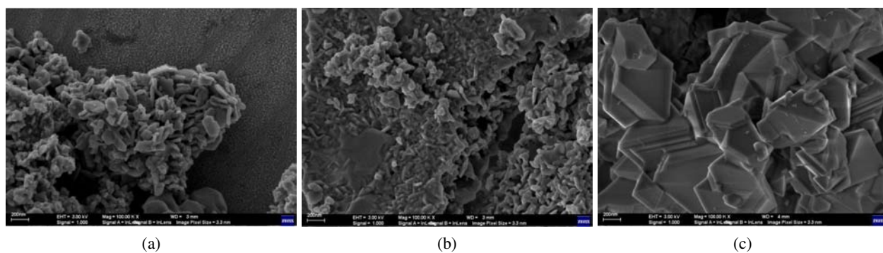
Figure 5. FEG-SEM of Y_3Fe_{5-x}Al_xO_{12} powders synthesized at 700\text{ }^\circ\text{C} for 2 h by the polymeric precursor method with: a) x = 1.5 , b) x = 1.6 and c) x = 1.7
