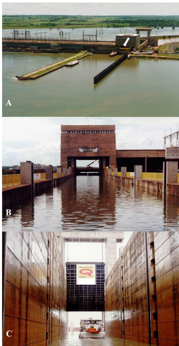
Figure 1. General view of the Jupiá Dam (A). It is possible to observe the location of the navigation lock in the dam (white arrow), and details of the floodgates up (B) and downstream (C). Credits: Companhia Energética de São Paulo – CESP.
