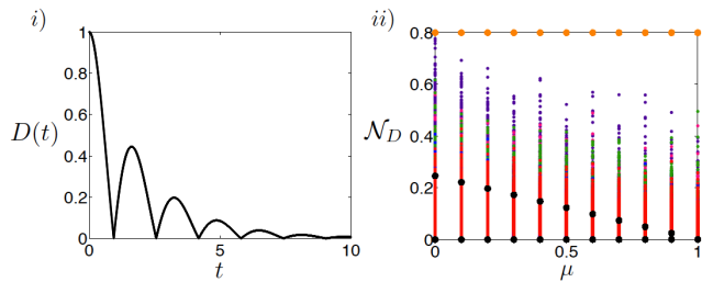
FIG. 1. a) Dynamics of the trace distance for the maximizing pair |\pm\rangle\langle\pm| for any value of the correlation parameter \mu , b) The BLP measure as a function of the correlation strength \mu for \tau = 1 . The following random states are present: maximally entangled states (purple), pure states (pink), mixed states (red) and product states (green), combinations of mixed and pure states (blue), Bell states (black crosses) and the product state |\pm\rangle\langle\pm| (orange stars). The optimal value is given by the highest point in the y-axis.
