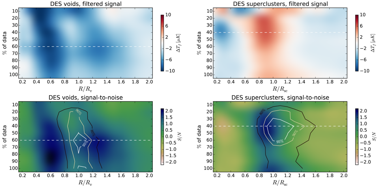
Figure 10. Top panels show stacked Planck CMB signals considering different data fractions and filter sizes, as for Jubilee in fig. 10. The top panels shows the stacked CMB imprint of DES Y1 voids and superclusters, while the bottom panels show the signal-to-noise ratios given the noise properties of the superstructures. We over plot contours obtained in the Jubilee analysis in order to show where the maximum S/N is expected. The dashed lines indicate the data fraction with highest S/N based on Jubilee, i.e. the one that we should a priori consider.
