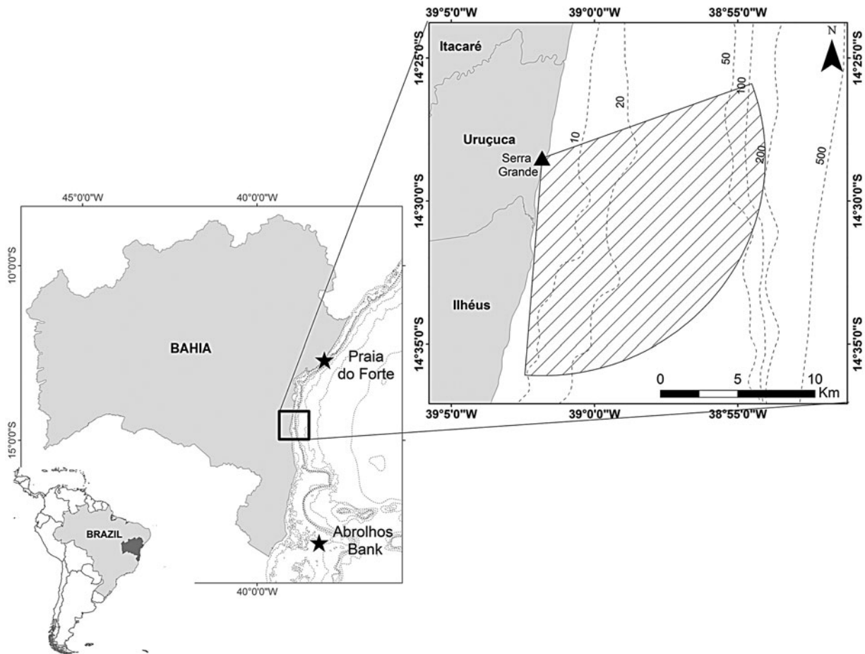
Fig. 1. Serra Grande study site located in north-eastern Brazil where a land-based observation station at elevation 93 m was used to conduct visual surveys that covered an area of 195.63 km 2 (striped area).
