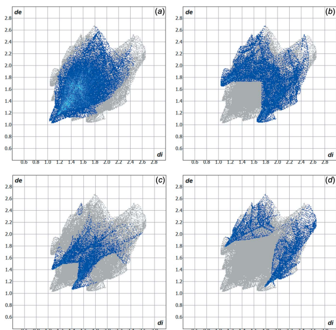
Figure 6 Hirshfeld surface two-dimensional fingerprint plots for the title compound showing the (a) \text{H}\cdots\text{H} , (b) \text{H}\cdots\text{C} , (c) \text{O}\cdots\text{H} and (d) \text{H}\cdots\text{S} contacts in detail (cyan dots). The contributions of the interactions to the crystal packing amount to 46.50, 23.40, 10.80 and 10.00%, respectively. The d_e ( y axis) and d_i ( x axis) values are the closest external and internal distances (values in Å) from given points on the Hirshfeld surface contacts.
