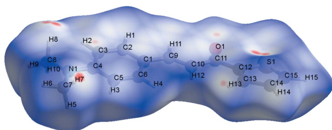
Figure 5 A graphical representation of the Hirshfeld surface ( d_{\text{norm}} ) for the title compound. The surface is drawn with transparency and all atoms are labelled. The surface regions with strongest intermolecular interactions for atoms H7, H8, H13 and O1, and for the thiophene ring, are shown in magenta.
