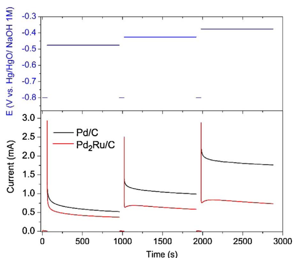
Fig. 9. Chronoamperometric profiles of Pd/C and Pd 2 Ru/C in 1.0 M NaOH solution containing 1.0 M ethanol.
