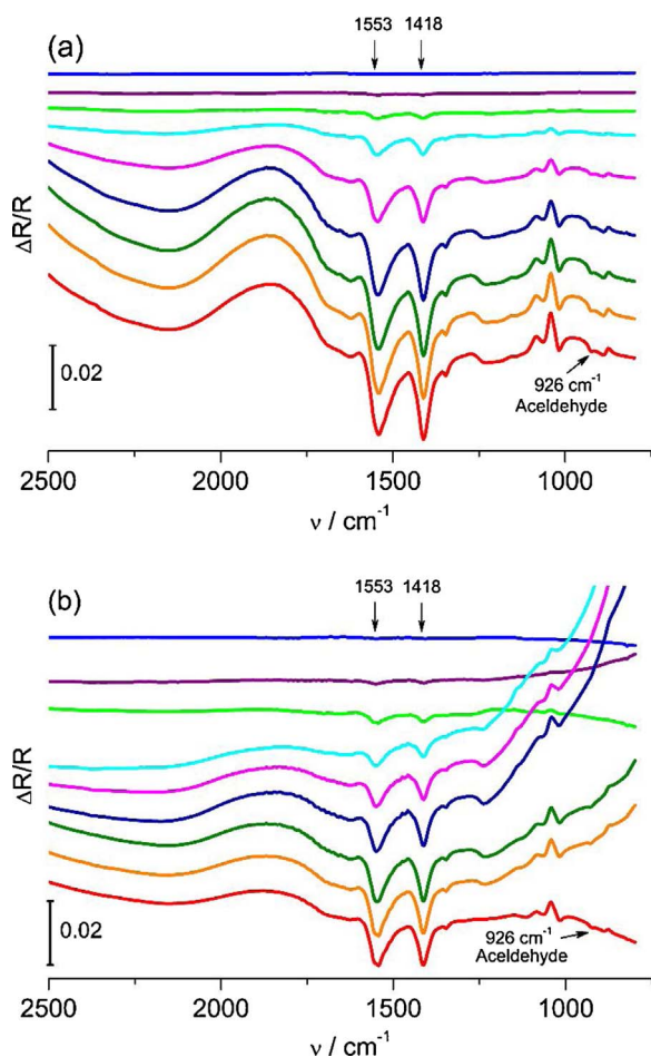
Fig. 10. In situ FTIR spectra of Pd/C (a) and Pd 2 Ru/C (b) electrocatalysts, ES was varied from -0.60 to 0.20 V, ER = -0.86 V vs. Hg/HgO/NaOH(1.0 M), 400 scans, 8 cm -1 . 1.0 M ethanol in 1.0 M KOH. Each spectrum corresponds to an increase of 0.1 V compared to the previous one.
