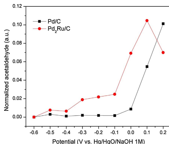
Fig. 11. Peak area of acetaldehyde band at 926 cm -1 normalized by ethanol oxidation current for the same amount of Pd loading vs. potential for Pd/C and Pd 2 Ru/C catalysts.
