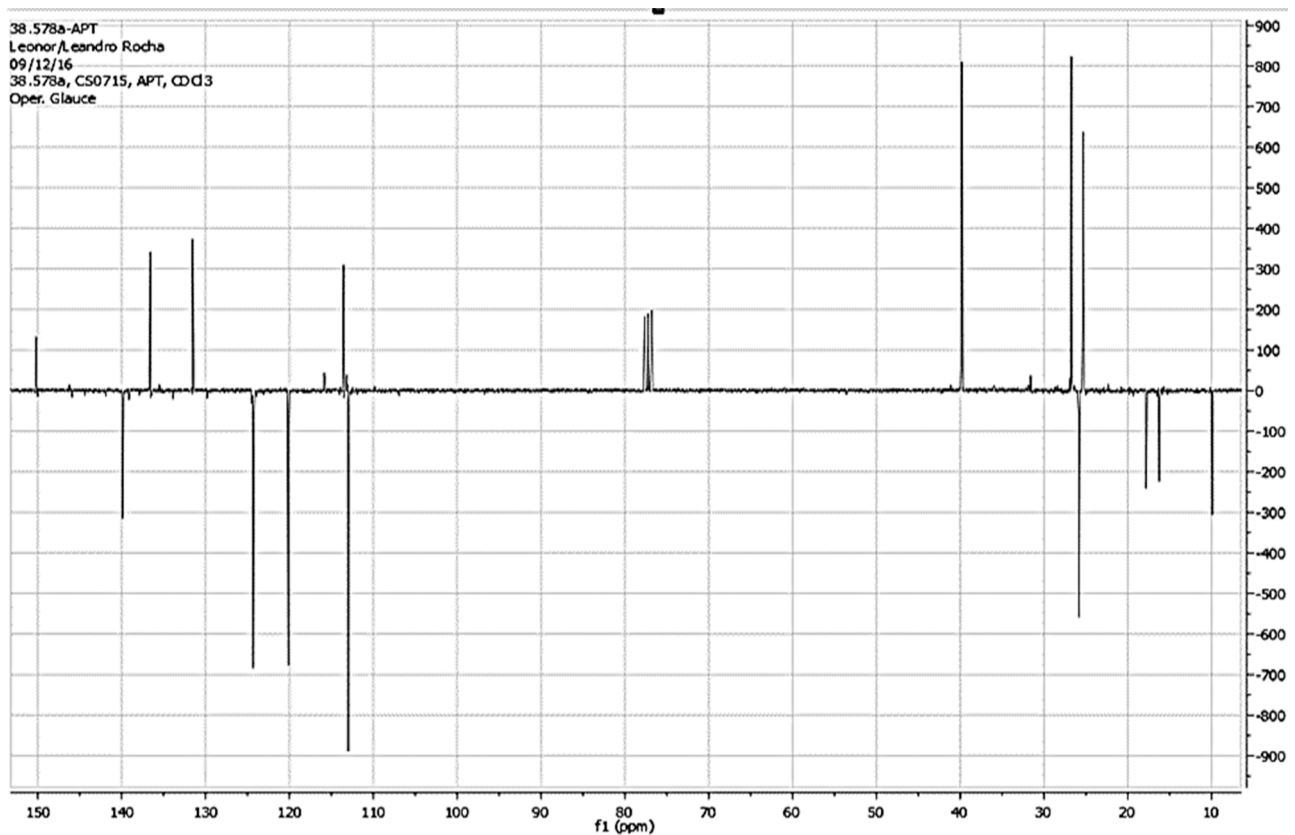
Fig. 1. NMR spectra of sesquirosefuran and its respective ^{13}\text{C} carbon chemical shifts (100 MHz, \text{CDCl}_3 ).
