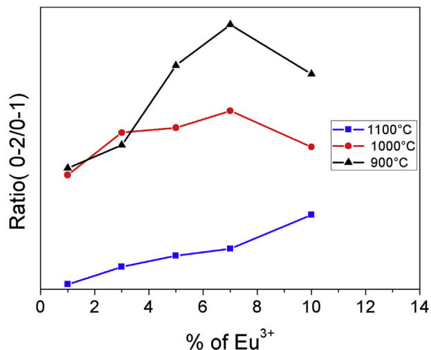
Fig. 10. Ratio between the integrated areas corresponding to the ^5D_0 \rightarrow ^7F_2 and D_0 \rightarrow ^7F_1 transitions of the Eu 3+ in CaYAIO 4 .
