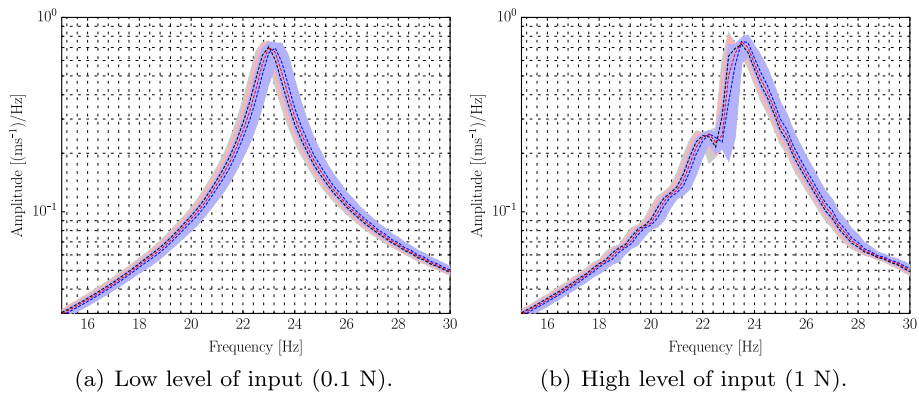
Fig. 8. FRFs considering different structural conditions and 2 levels of input amplitude. ■ represents \alpha = 1 (reference condition), ■ \alpha = 0.98 (damaged condition) and ■ \alpha = 0.96 (damaged condition).
