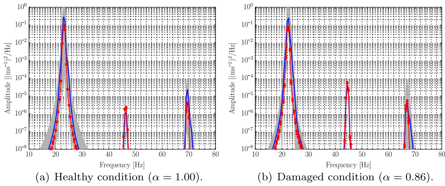
Fig. 11. Stochastic Volterra model response in comparison with new simulated data, in frequency domain, considering a single tone sine input and two structural conditions. The gray box represents the 99% confidence bands, — represents the mean and — o — the simulated data.
