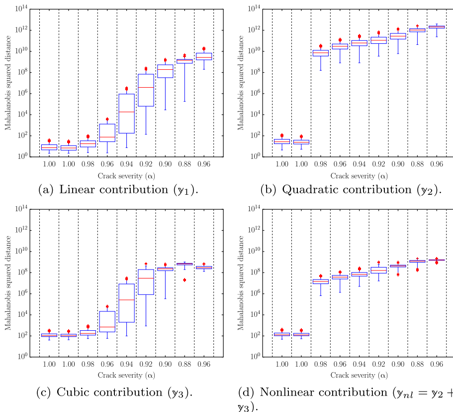
Fig. 16. Boxplot of Mahalanobis squared distance of the kernels contribution calculated for different levels of crack severity.
