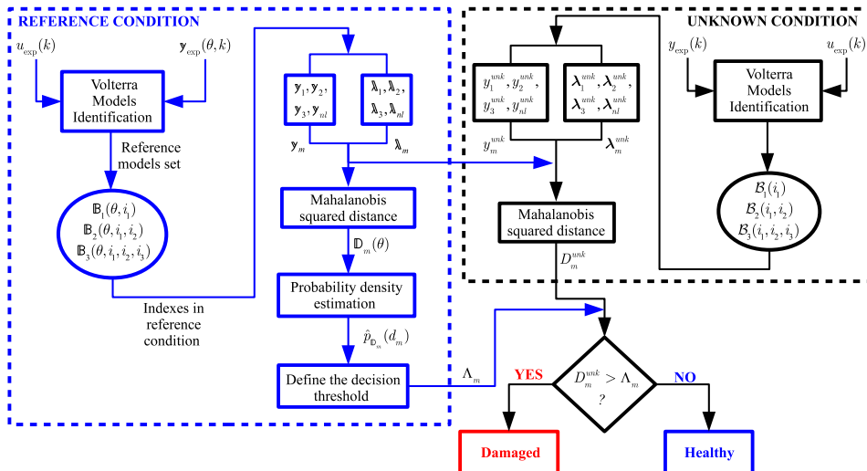
Fig. 2. Description of the damage detection approach based on stochastic Volterra series.
