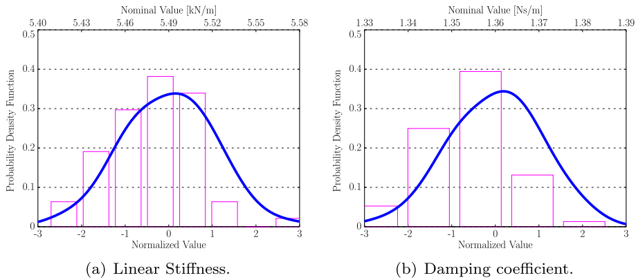
Fig. 7. Distribution of the random parameters k_1 and c .
