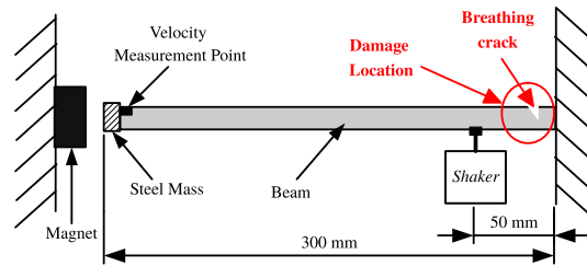
Fig. 5. Nonlinear system simulated in the damaged condition.
