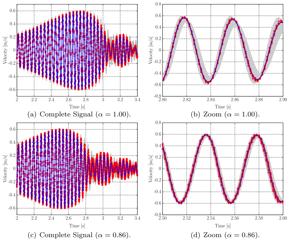
Fig. 10. Stochastic Volterra model response in comparison with new simulated data, considering a high level amplitude chirp input (1 N) and two structural conditions. The gray box represents the 99% confidence bands, — represents the mean and —○— the simulated data.
