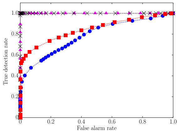
Fig. 15. Receiver operating characteristics (ROC) curve, obtained using the kernels coefficients. ● represents the linear index, × the quadratic index, ■ the cubic index and ▲ the nonlinear index.
