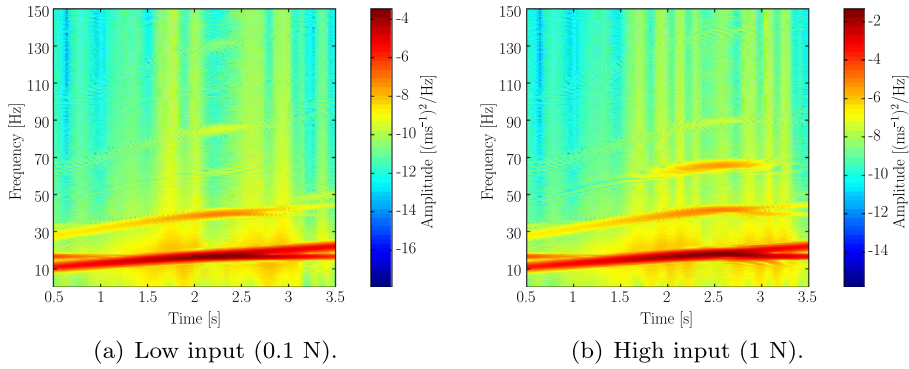
Fig. 6. Time–frequency diagram of the response for different levels of input amplitude, considering the crack severity \alpha = 0.9 .
