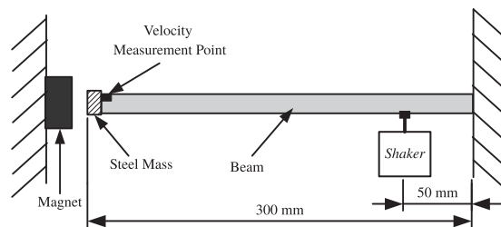
Fig. 3. Nonlinear system simulated in the reference condition.
