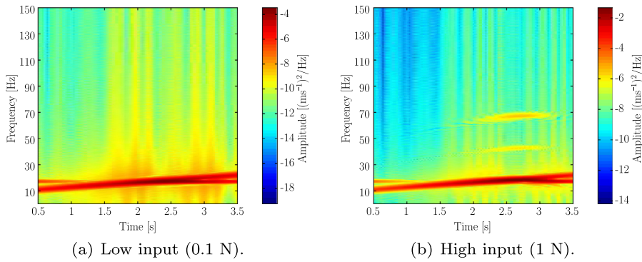
Fig. 4. Time–frequency diagram of the response for different levels of input amplitude, considering the reference condition (Healthy).
