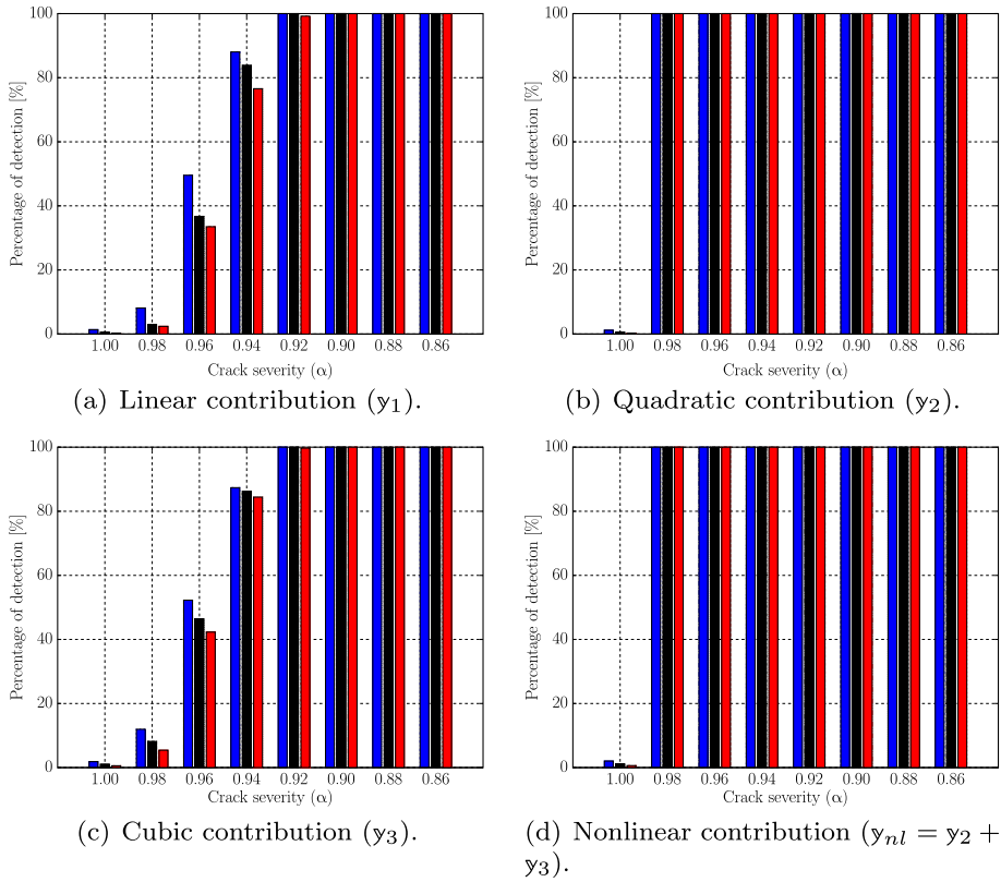
Fig. 17. Percentage of damage detection obtained using the kernels contribution, considering different crack severities and probability of false alarms used. ■ represents \beta = 0.02 , ■ represents \beta = 0.01 and ■ represents \beta = 0.005 .
