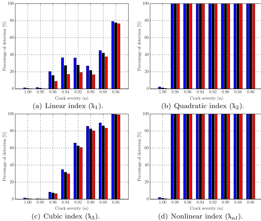
Fig. 14. Percentage of damage detection obtained using the kernels coefficients, considering different crack severities and probability of false alarms used. ■ represents \beta = 0.02 , ■ represents \beta = 0.01 and ■ represents \beta = 0.005 .
