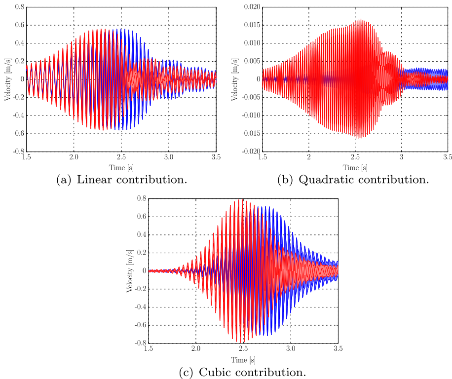
Fig. 12. Confidence bands of the kernels contribution to the total system response obtained through the Volterra model with 99% of confidence, considering high level of input (1 N). ■ represents the reference condition ( \alpha = 1.00 ) and ■ the damaged condition ( \alpha = 0.86 ).
