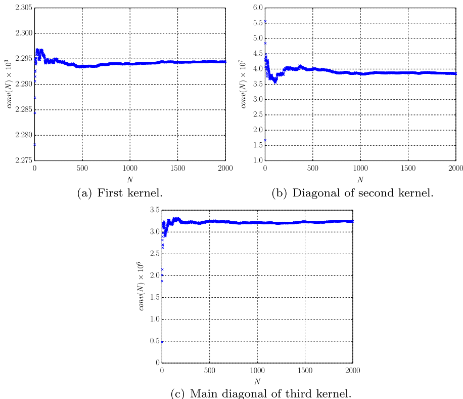
Fig. 9. MC convergence test applied to the Volterra kernels identified in the reference condition ( \alpha = 1.00 ).
