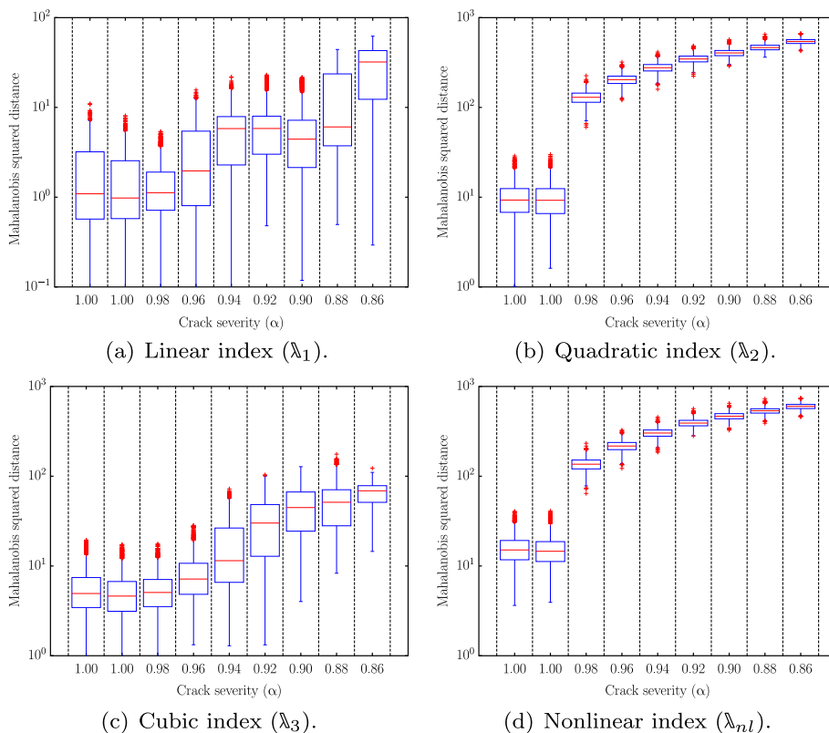
Fig. 13. Boxplot of the Mahalanobis squared distance applied to the four indexes calculated, for different levels of crack severity.
