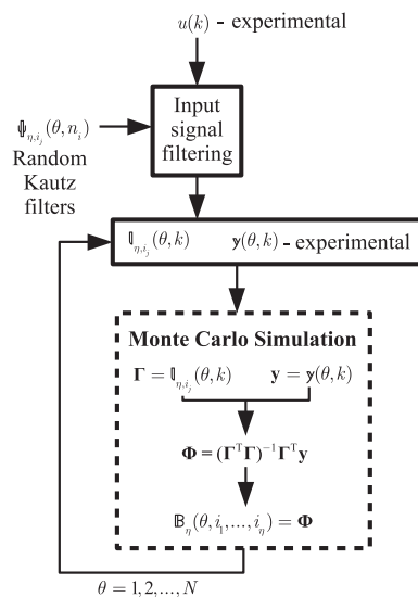
Fig. 1. Description of the Volterra kernels identification approach used, based on Monte Carlo simulations.
