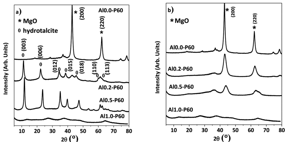
Fig. 3 X-ray diffractograms of the Al–Mg mixed oxides with different aluminum mole fractions: (a) reconstructed hydrothermal samples exposed to room atmosphere; (b) samples calcined at 500 °C and measured immediately.
