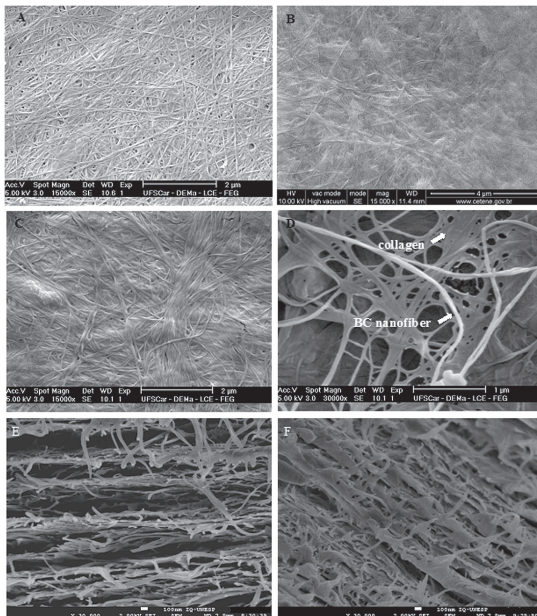
Figure 1. SEM surface images of the BC, BC-COL and BC-COL OGP(10-14) membranes ((A)–(C), respectively; 15 000 \times ); BC-COL OGP(10-14) membrane ((D), 30 000 \times ). SEM cross-section images of the BC and BC-COL OGP(10-14) membranes ((E) and (F), respectively; 30 000 \times ).
