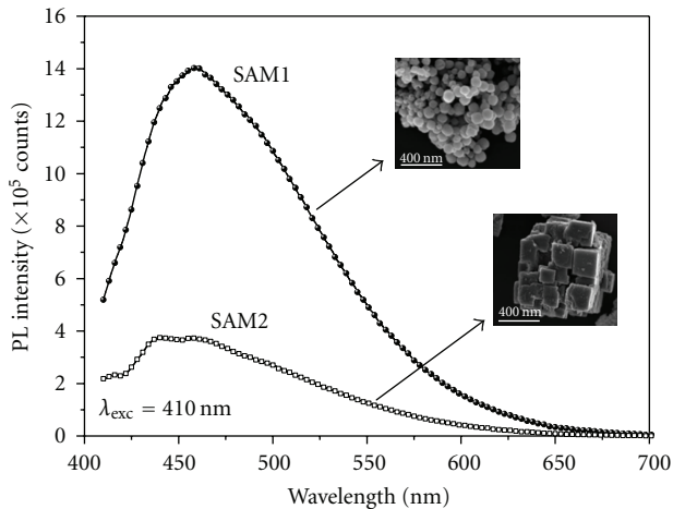
FIGURE 4: Room temperature photoluminescence spectra of SrTiO 3 samples with different shapes.
