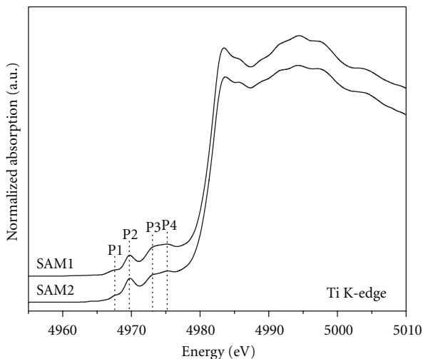
FIGURE 5: Ti K-edge XANES spectra of SrTiO 3 samples.
