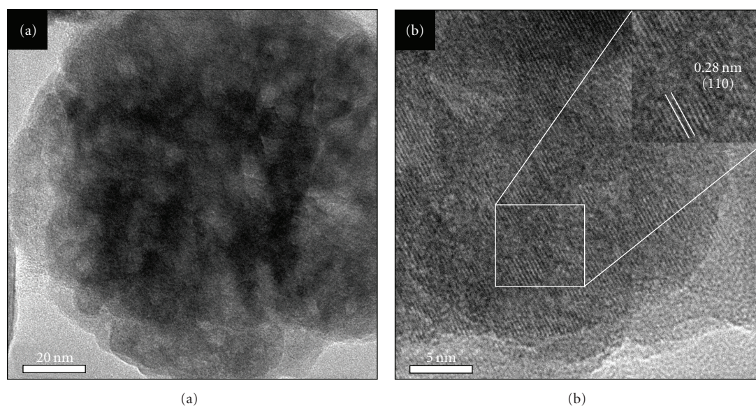
FIGURE 3: (a) TEM and (b) HR-TEM images of the SAM1 sample.
