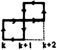
FIG. 2. A loop giving a vanishing contribution to the phase of S_{mn} .
