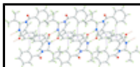
Fig. 2. Supramolecular chain in (I) comprising centrosymmetric dimers mediated by \{O=C—N—H\cdots\}_2 synthons (hydrogen bonds shown as orange dashed lines) linked by C—H\cdots\pi interactions (shown as purple dashed lines).
