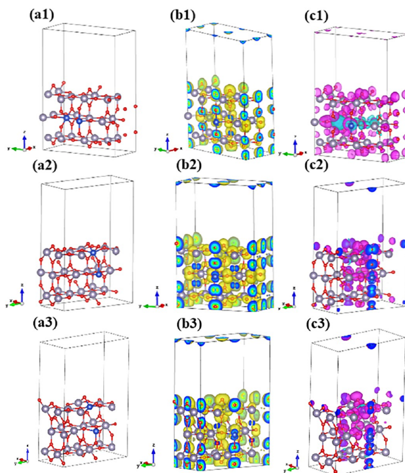
Figure 3. 2D bulk structures with two substitutional Cu atoms, within deep in plane ( dlp ) (a1), and belonging to the two neighboring planes ( pp ), one in the surface and other in subsurface plane (a2), and corresponding local density of states (LDOS) (b1, b2), and spin-charge density difference (SCHDD) (c1, c2).
