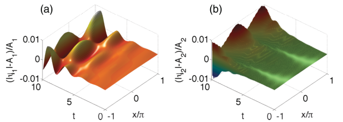
FIG. 2. (Color online) Solutions to the full PDE model of Eq. (1) for driven coupling between fermions and bosons with the modulation frequency \Omega_{12,+} = 65.5 ( k = 1 ). We plot the oscillating parts (|\psi_j| - A_j)/A_j for (a) j = 1 (bosons) and (b) j = 2 (fermions). The initial conditions are \psi_j = A_j[1 + 10^{-4} \exp(ikx)] and the boundary conditions in x are periodic. The parameters are the same as in Fig. 1.
