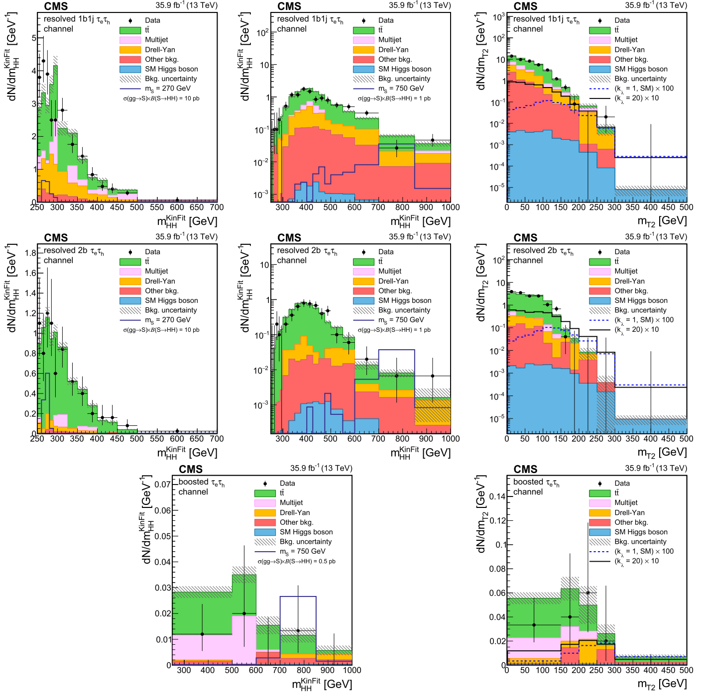
Fig. 3. Distributions of the events observed in the signal regions of the \tau_e \tau_h final state. The first, second, and third rows show the resolved 1b1j, 2b, and boosted regions, respectively. Panels in the right column show the distribution of the m_{T2} variable, while the other panels show the distribution of the m_{HH}^{\text{KinFit}} variable, separated in the low-mass (LM, left panels) and high-mass (HM, central panels) regions for the resolved event categories. Data are represented by points with error bars and expected signal contributions are represented by the solid (BSM HH signals) and dashed (SM nonresonant HH signal) lines. Expected background contributions (shaded histograms) and associated systematic uncertainties (dashed areas) are shown as obtained after the maximum likelihood fit to the data under the background-only hypothesis. The background histograms are stacked while the signal histograms are not stacked.
