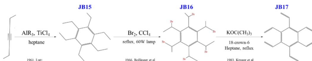
Figure 60 -Synthesis of the molecule JB17 via known steps [cxxxi,cxxxii].
