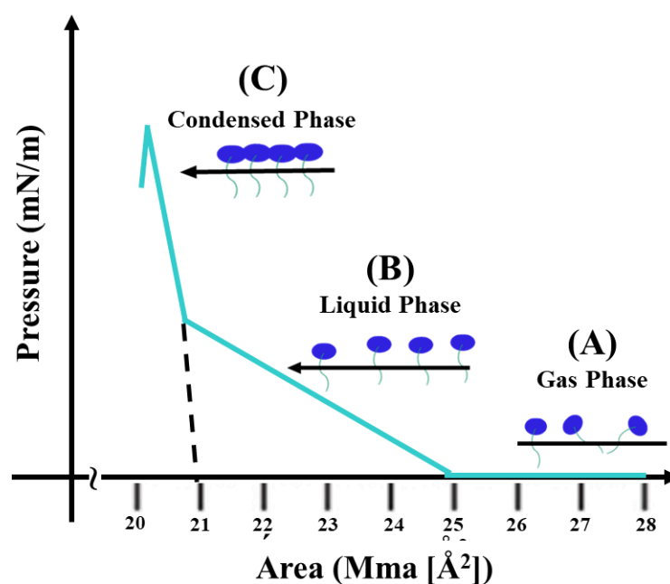
Figure 18 -Isothermal \pi -A for stearic acid[113].
