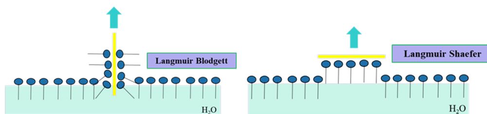
Figure 19 -Langmuir-Blodgett (a) and Langmuir-Schaefer (b) deposition scheme.
