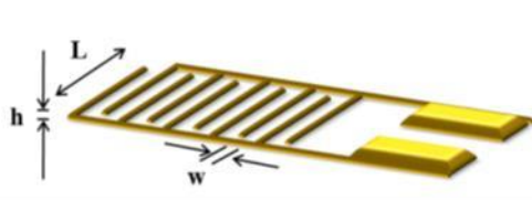
Fig A2 - IDE representation with N = 10 digits, h height, L length and w digit width, dimensions 110 nm high ( h ), 8 mm long ( L ) and 100 \mu\text{m} wide ( w ).
