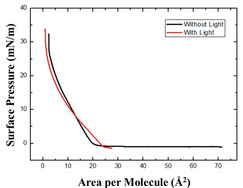
Figure 61 -Pressure area isotherms curves of the molecule 4 (black) without and (red) with light showing no change beyond that of experimental error and indicating that no reaction had occurred when light had been put on the molecule JB17
