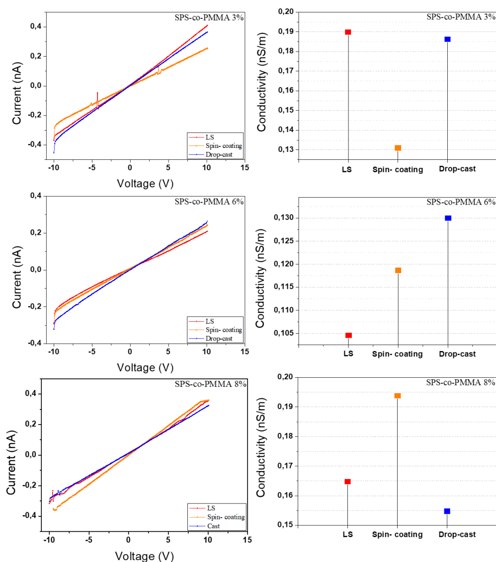
Figure 28- I versus V graph and DC electrical conductivity of LS films, spin-coating and drop-cast of SPS-co-PMMA 3, 6 and 8% ionomers.
