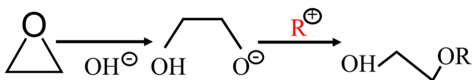
Figure 9 -The polymerization reaction leading to poly(ethylene oxide). The metallic ion, typically, \text{Na}^+ , \text{K}^+ or \text{Cs}^+ is not shown for simplicity.
