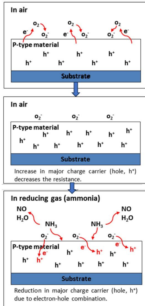
Figure 14- Sensing mechanism of p-type material in air and reducing gas environments.[96].
