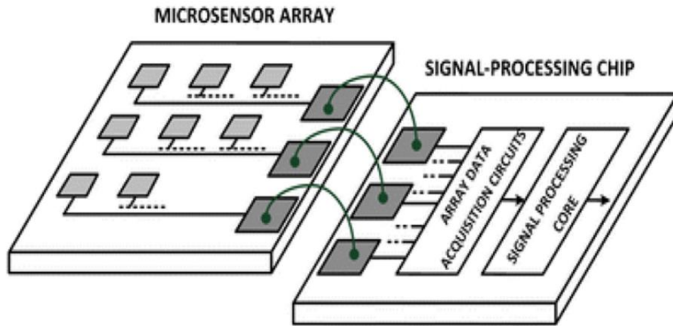
Figure 11 -A two-chip solution for E-nose system, comprising a front-end sensor array and a back-end low-power signal-processing chip in 2014[67]
