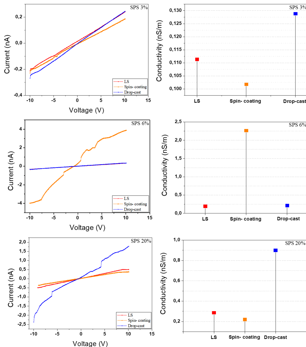
Figure 29 -Graph IxV and DC electrical conductivity of LS films, spin-coating and drop-cast of SPS 3, 6 and 20% ionomers.
