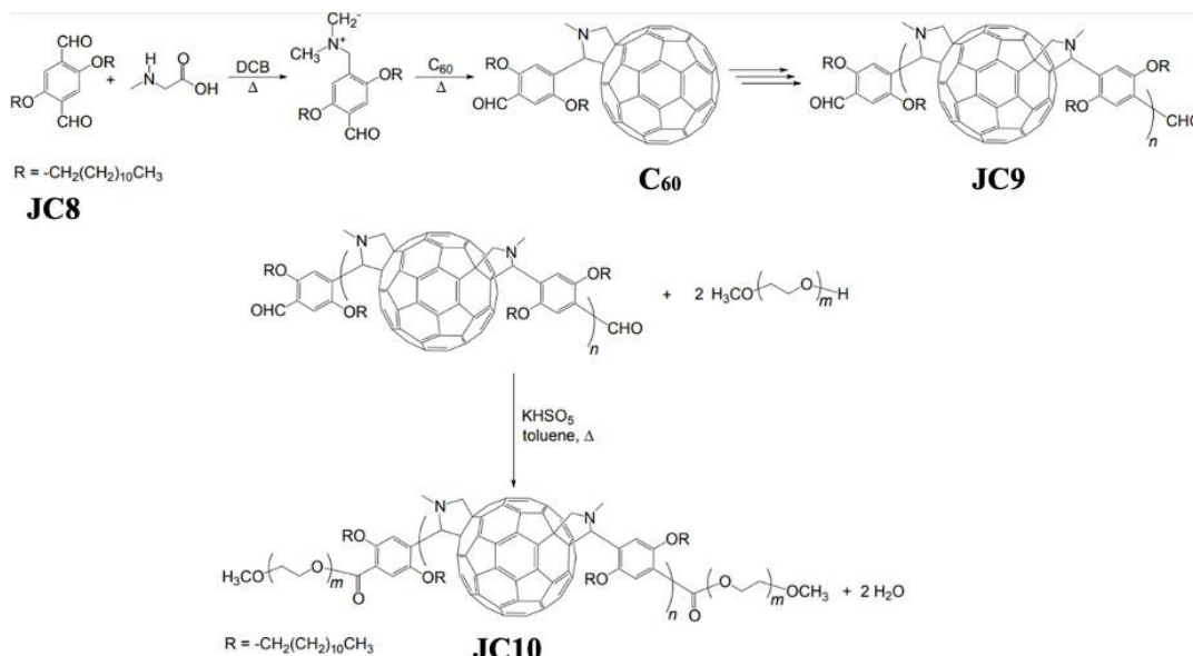
Figure 40 -Chemical structure of block copolymer poly[fullerene-alt-(2,5-bisdicyloxy-1,4-terephthaldehyde)]-block-poly(ethylene oxide) ( JC10 )
