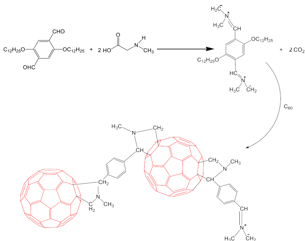
Figure 50 -Aproposed mechanism for the synthesis of JC9, where the azomethine ylide is formed before the reaction with the C60.
