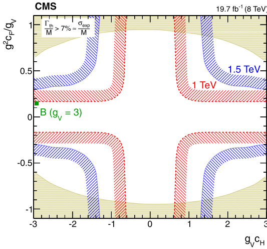
Fig. 7. Exclusion regions in the plane of the HVT-model coupling constants ( g_{VC_H} , g^2 C_F / g_V ) for two resonance masses, 1.0 and 1.5 TeV. The point B of the benchmark model used in the analysis, corresponding to g_V = 3 and C_F = -C_H = 1 , is also shown. The boundaries of the regions of the plane excluded by this search are indicated by the dashed and dotted lines, and associated hatching. The areas indicated by the solid line and solid shading correspond to regions where the theoretical width is larger than the experimental resolution of the present search and thus the narrow-resonance assumption is not satisfied.
