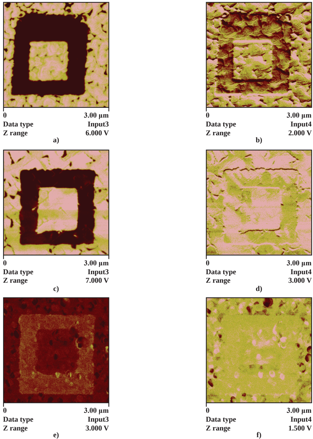
Figure 6. Out-of-plane (OP) and In-plane (IP) PFM images of BZT10:2V ceramics sintered at 1200°C for 2 hours in a conventional furnace. (a) OP ( N_2 ) and (b) IP ( N_2 ), (c) OP ( O_2 ) and (d) IP ( O_2 ), (e) OP ( At_{amb} ) and (f) IP ( At_{amb} )
