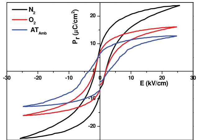
Figure 4. Hysteresis loops for BZT10:2V ceramics sintered at 1200°C for 2 hours in a conventional furnace under \text{N}_2 , \text{O}_2 and \text{At}_{\text{amb}} atmospheres
