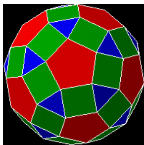
Figura 44: Poliedro (3,4,5,4)
