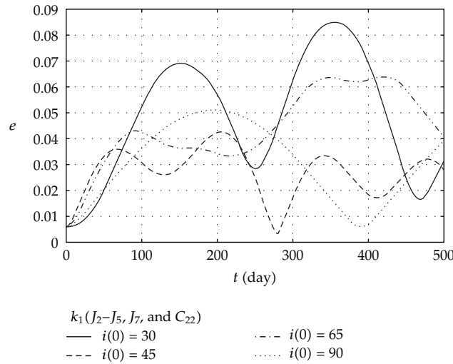
Figure 15: LP165P Model, e = 0.006 , g = 270^\circ , and h = 90^\circ .
