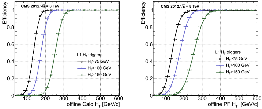
Figure 39. The L1 H_T efficiency turn-on curves as a function of the offline CaloJet (left) and PF (right) H_T , for three thresholds ( H_T > 75, 100, 150 GeV).
