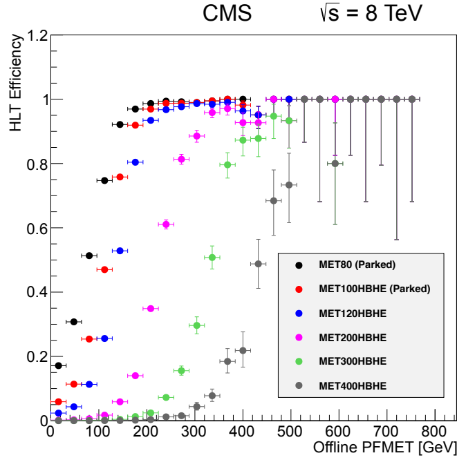
Figure 44. The HLT efficiencies as a function of the offline PF E_T^{\text{miss}} for different E_T^{\text{miss}} thresholds ( E_T^{\text{miss}} = 80\text{--}400\text{ GeV} ).
