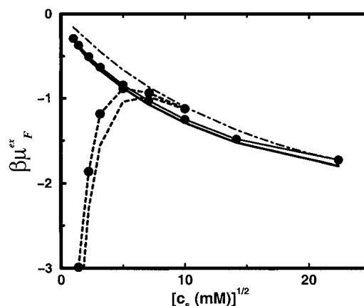
Fig. 2. The reduced excess chemical potential for a free divalent cation in a 20 \mu M protein solution is indicated as a function of monovalent salt concentration. The (superimposed) solid lines refer to the SC8 model and the broken lines to the SC24 model. Lines marked by solid circles are calculated with a dielectric boundary radius R_d = 14 Å; lines without symbols refer to R_d = 0 Å. The thin broken line shows the excess chemical potential of a divalent ion in a bulk salt solution.
