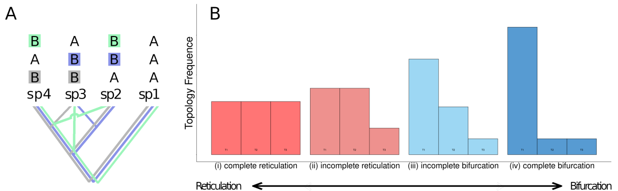
Figure 1. Distribution of bi-allelic patterns along the reticulation-bifurcation continuum and the 2A2B test. A) The distribution of bi-allelic sites of four species can generate three distinct topologies, BBAA with sp.3 and sp.4 as sister (gray topology), ABBA with sp.2 and sp.3 (blue topology) and BABA with sp.2 and sp.4 are most closely related (green topology). B) Based of the frequency of these topologies in a genome fragment, this fragment can be categorized in (i) complete reticulation, T1=T2=T3 (, (ii) incomplete reticulation, T1=T2>T3 , (iii) incomplete bifurcation, T1>T2>T3 , and (iv) complete bifurcation, T1>t2=T3 , these classes are shown in red, pink, light blue and blue, respectively.
