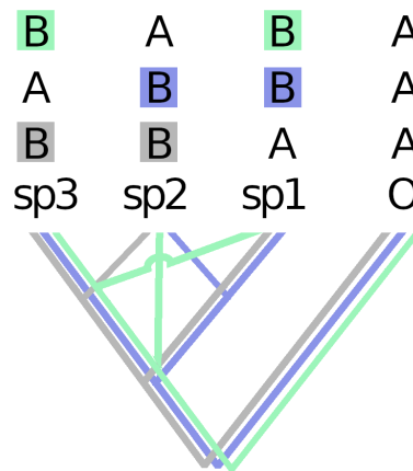
Figure 1. Potential topological structures in species quartets with an outgroup, inferred from shared genetic variation in Pairs. Three Distinct Topologies are possible: AABB (gray, species 2 and 3 as the closest relatives), ABBA (blue, species 1 and 2 as the most closely related), and BABA (green, species 1 and 3 as the nearest pair).
