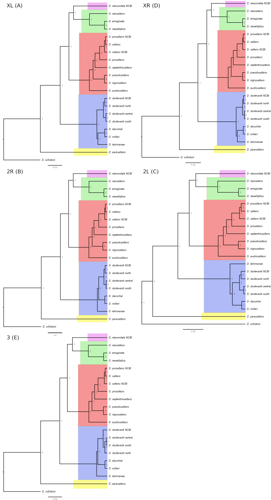
Supplementary Figure S1. Bayesian Inference trees generated with 5 independent datasets, chromosome arms and respective Muller elements are indicated in each tree. Branch Posterior probabilities are shown for each node. The parasaltans , sturtevantii , saltans , elliptica and cordata subgroups are highlighted in yellow, blue, red, green and pink, respectively.
