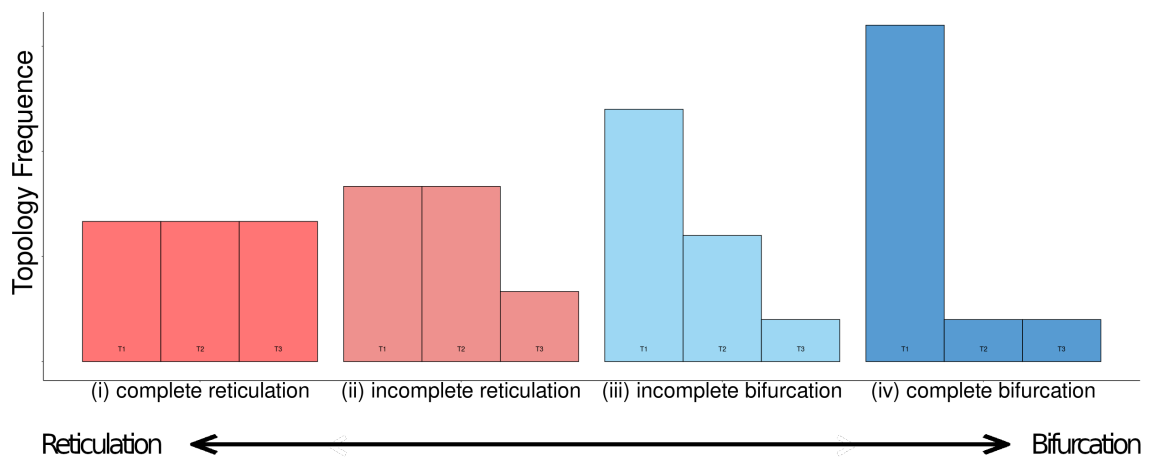
Figure 2. Four possible classes of topological frequency distributions across the genome. These classes offer insights into diverse evolutionary scenarios: class I, complete reticulation, expected in genome regions impacted by ILS; class II, bidirectional exchange of genetic material, interpreted as a signal of hybridization; class III, asymmetric exchange of genetic material, interpreted as introgression; and class IV, complete bifurcation, expected in events of speciation without ILS and gene flow.
