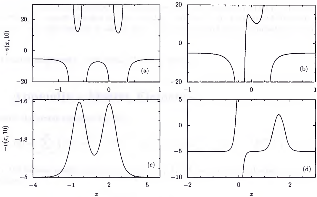
Figure 2: 2-soliton solutions for eqn. (2.21). v_0 = 5 and t_{-2} = 10 . Parameters: (a) \gamma_1 = -4 , \gamma_2 = -3 ; (b) \gamma_1 = -4 , \gamma_2 = -10 ; (c) \gamma_1 = 1.3 , \gamma_2 = 1.5 ; (d) \gamma_1 = 4.8 , \gamma_2 = 7 .
