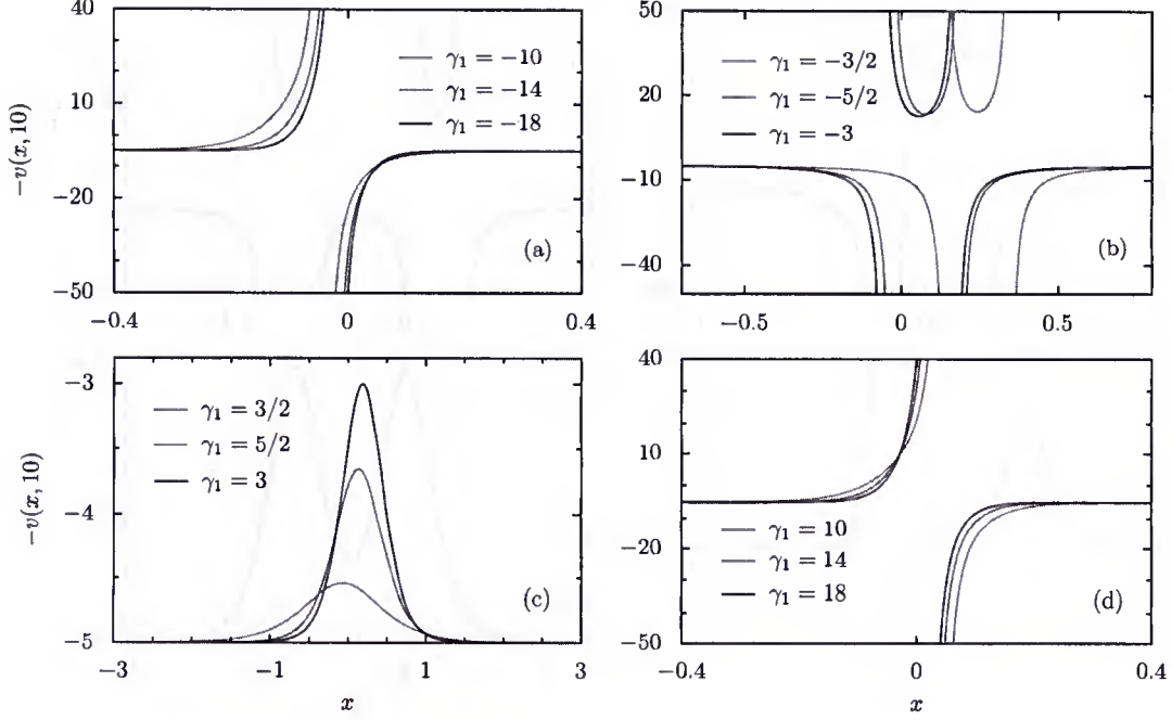
Figure 1: 1-soliton solutions for eqn. (2.21), t_n = t_{-2} in mKdV hierarchy. In all these graphs we set v_0 = 5 and choose a fixed time t_{-2} = 10 .
