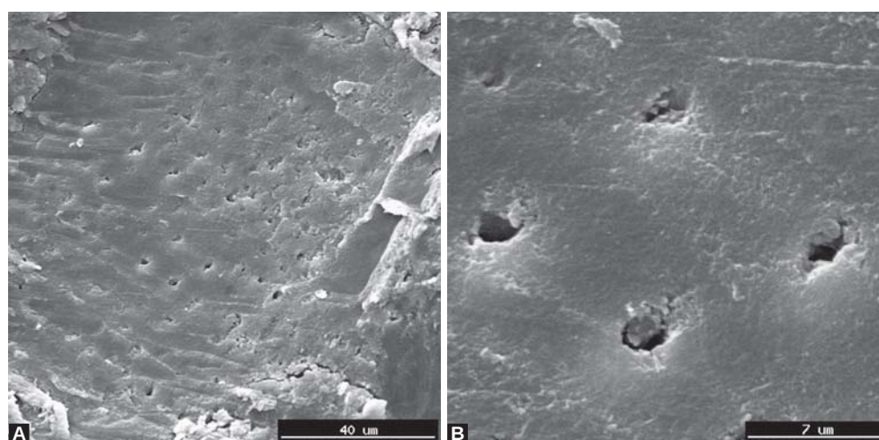
Figs 2A and B: (A) Surface prepared with CVD tip (1000 \times ); (B) 5000 \times . Dentin tubules partially opened and small quantity of smear layer
