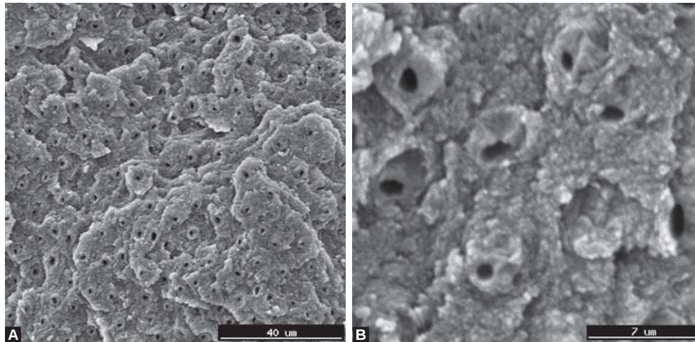
Figs 3A and B: (A) Surface prepared with Er:YAG laser (1000×), (B) 5000×. Presence of opened tubules and absence of smear layer
