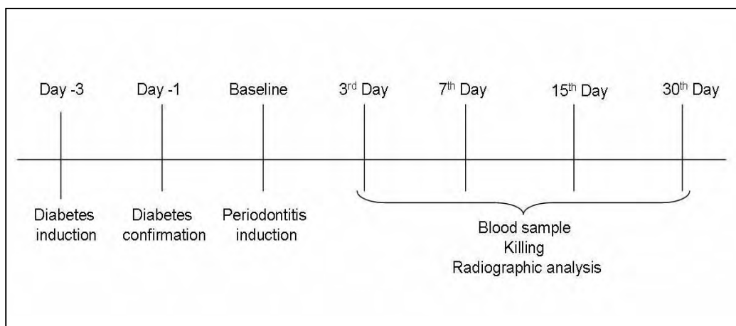
Figure 1 Experimental chronology.
