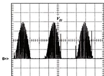
Escala vertical: V_{S1} : 100 V/div Escala horizontal: 5 ms/div; (a) S_1
