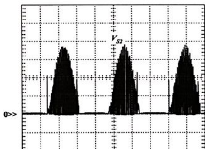
Escala vertical: V_{S2} : 100 V/div Escala horizontal: 5 ms/div; (a) S_2
