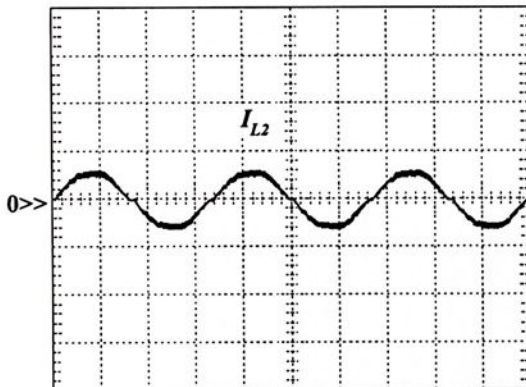
Escala vertical: I_{L2} : 5 A/div Escala horizontal: 5 ms/div; (a) I_{L2}
