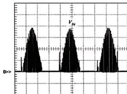
Escala vertical: V_{S4} : 100 V/div Escala horizontal: 5 ms/div; (b) S_4
