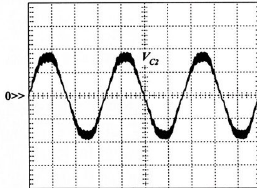
Escala vertical: V_{C2} : 100 V/div Escala horizontal: 5 ms/div; (a) V_{C2}
