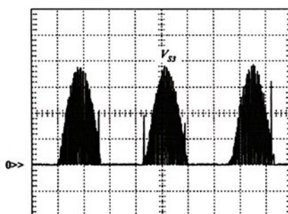
Escala vertical: V_{S3} : 100 V/div Escala horizontal: 5 ms/div; (b) S_3
