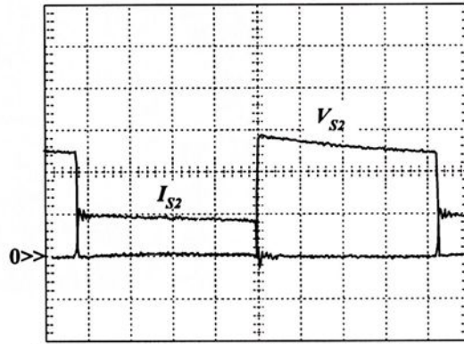
Escala vertical: V_{S2} : 100 V/div; I_{S2} : 5 A/div Escala horizontal: 3,5 ms/div; (a) V_{S2} e I_{S2}
