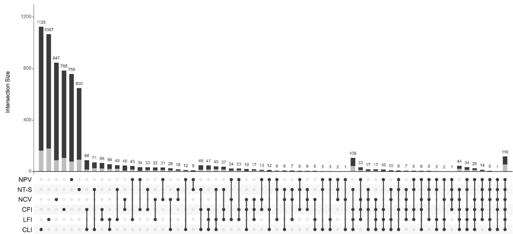
Figure 4. UpSet plot composed of OTUs present in the different production systems at Barbosa farm, Brejo, Maranhão, Brazil, 2022. Circles indicate the system. Lines connecting the circles indicate sharing between systems. Stacked bars indicate the size of the intersection (number of OTUs) for each set, where light gray bars represent OTUs with identification up to the genus level, while the black portion indicates OTUs not classified to genus.
