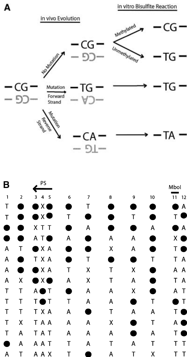
Figure 1. Direct DNA sequencing of bisulfite repetitive element PCR of Alu elements. (A) Schematic of possible fates of Alu element CpG methylation sites. Due to the mutation of CpG sites via spontaneous deamination of 5-methylcytosine to T during evolution, a CpG site can be changed into a TpG or CpA dinucleotide. Neither TpG nor CpA are targets for methylation. Following bisulfite treatment, a methylated CpG will remain CpG. However, an unmethylated CpG will give rise to TpG, which is indistinguishable from a deamination mutation of the forward strand. Thus, three possibilities arise for our sequencing data: CpG that represents a methylated CpG site, TpG that represents either an unmethylated CpG site or a mutation of the forward strand, and TpA that represents a mutation of the reverse strand followed by conversion of the unmethylated C to T by bisulfite. (B) Sequencing data of bisulfite repetitive element PCR of Alu elements. Genomic DNA was isolated from peripheral human blood and bisulfite treated. Alu element PCR was performed and the PCR product was cloned, and 15 clones were sequenced. There were 12 potential CpG methylation sites per clone for a total of 180 potential methylation sites sequenced. Black circles represent methylated CpG sites (66/180 = 36.7%). 'T' represents TpG sites that were either unmethylated or mutated (53/180 = 24.4%). 'A' represents TpA sites that were mutated (41/180 = 22.8%). 'X' represents other mutations (20/180 = 11.1%). The CpG sites used for pyrosequencing ('PS') and COBRA ('MboI') are indicated.
