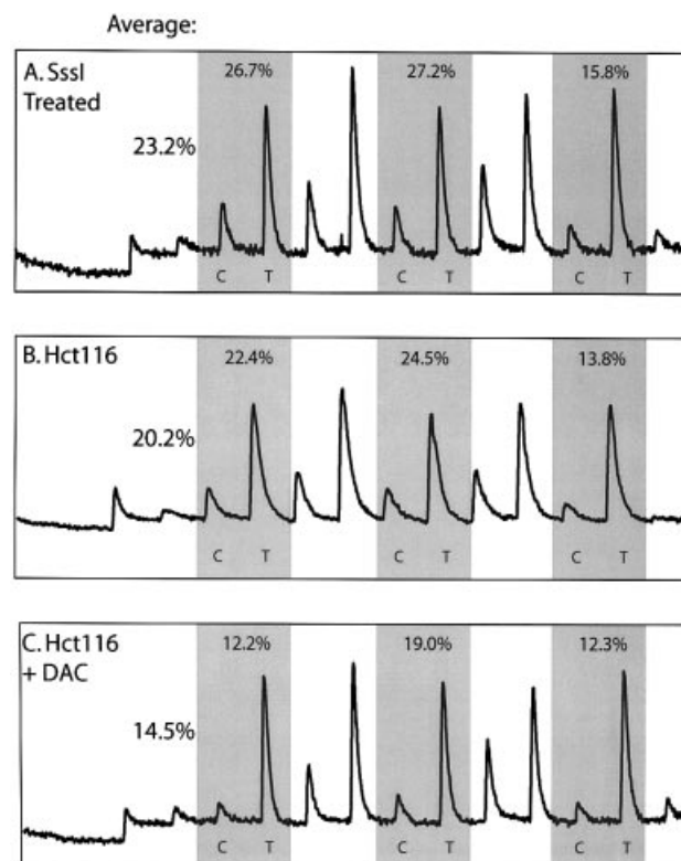
Figure 4. Quantitation of DNA methylation using bisulfite repetitive element PCR and pyrosequencing. (A) SssI methylase-treated DNA, (B) untreated Hct116 cell line DNA or (C) DAC-treated Hct116 cell line DNA was bisulfite treated and PCR of Alu repetitive elements was performed. The PCR product was purified and methylation was quantitated using the PSQ HS 96 Pyrosequencing System (Pyrosequencing, Inc.). The pyrogram quantitates C for methylated and T for unmethylated or mutated DNA. The shaded regions represent three tandem CpG sites quantitated in Alu elements, and the percent methylation at each site is shown above the peaks. The average methylation of the three sites is calculated on the left for each pyrogram. The maximum absolute methylation of 23.2% is calculated by SssI methylase-treated DNA (A), Hct116 cells have 20.2% methylation, and this methylation decreases to 14.5% after DAC treatment of Hct116 cells.
