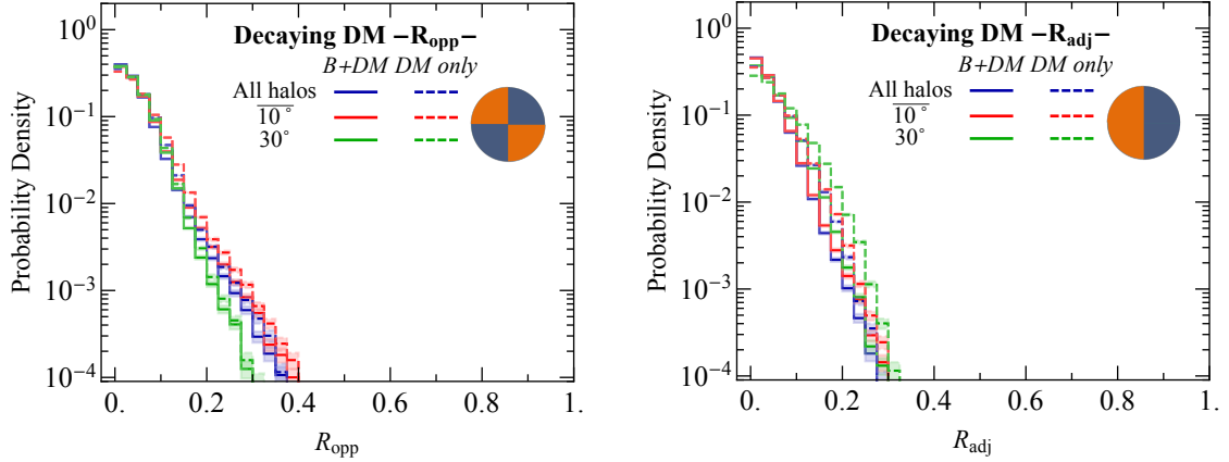
Figure 13. As figure 3, except for decay rather than annihilation.
