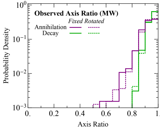
Figure 5. Histogram of the observed axis ratio for annihilation and decay of MW-like halos as defined by the requirements in eqs. (3.2) and (3.3). The distribution of the MW-like halos is shown in solid lines while the distribution of rotated halos to increase statistics is shown in dotted lines.
