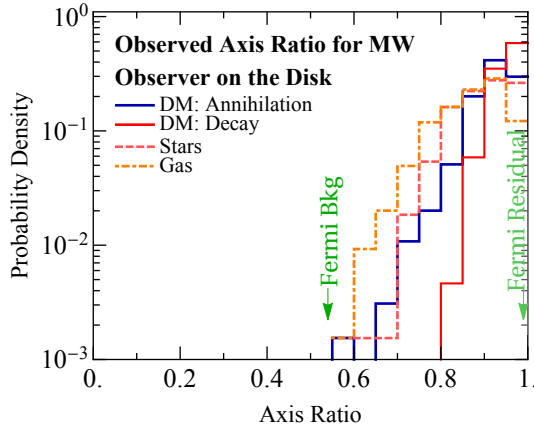
Figure 11. Histogram of the observed axis ratio for annihilation and decay of DM in MW-like halos as defined by the requirements in eqs. (3.2) and (3.3). We also show the histograms of the distribution of gas and stars, computed in similar manner as DM decay. We finally show the axis ratio of the Fermi background data, as well as the residual Fermi signal as discussed in section 5.1.
