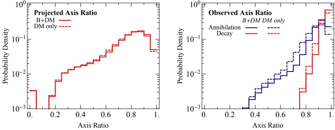
Figure 2. Histogram of the conventional 2-dimensional axis ratio (left) and the newly defined observed axis ratio (right) for annihilation and decay, comparing both Illustris-1 and Illustris-1-Dark (see eq. (2.6)).
