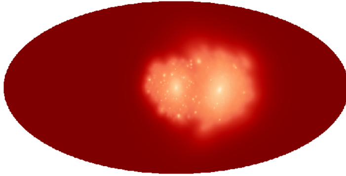
Figure 9. Logarithmic map for DM annihilation for halo labeled “499” in the Illustris-1 simulation from the point of view of an observer external to the halo. We used HEALPix with n_{\text{side}} = 512 (see eq. (2.4)). The observer is located at a distance 2R_{200} = 478 kpc of the center. The halo mass is 2.72 \times 10^{12} M_{\odot} .
