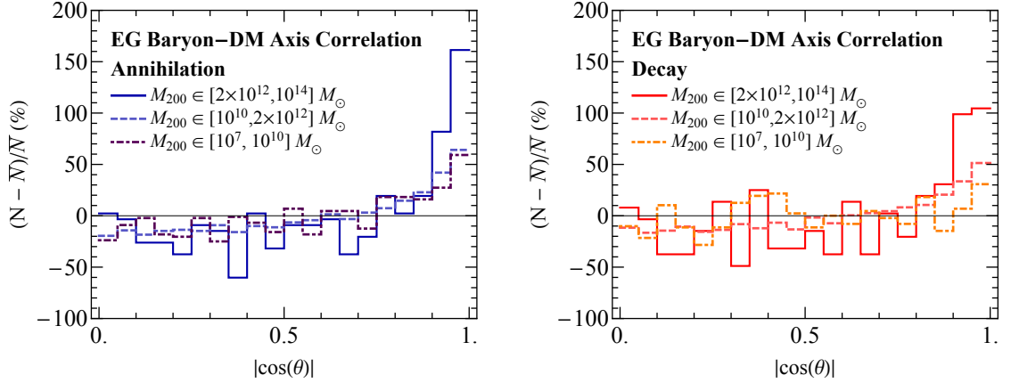
Figure 16. Histograms of the angle between the halo's minor axis and the angular momentum vector of the baryons in annihilation (left) and decay (right) for three different mass bins: M_{200} > 2 \times 10^{12} M_{\odot} , 10^{10} M_{\odot} < M_{200} < 2 \times 10^{12} M_{\odot} and M_{200} < 10^{10} M_{\odot} .
