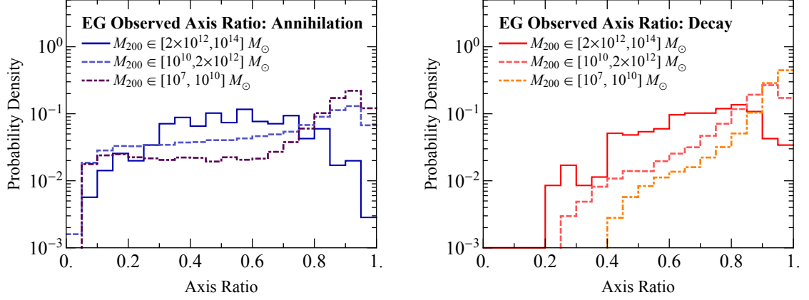
Figure 15. Histograms of the observed axis ratio for annihilation (left) and decay (right) for different mass bins: M_{200} > 2 \times 10^{12} M_{\odot} , 10^{10} M_{\odot} < M_{200} < 2 \times 10^{12} M_{\odot} and M_{200} < 10^{10} M_{\odot} .
