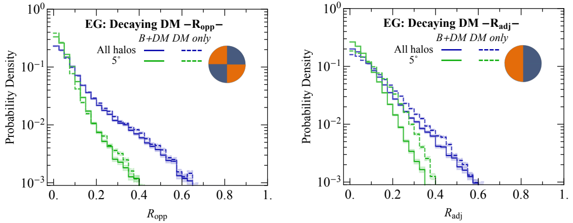
Figure 14. As figure 7, except for decay rather than annihilation.
