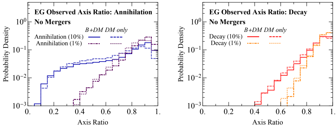
Figure 10. Histogram of the newly defined observed axis ratio for annihilation and decay for extragalactic sources, comparing both Illustris-1 and Illustris-1-Dark (see eq. (2.6)) after having omitted the “merger” halos (see text).
