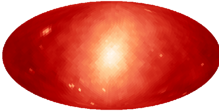
Figure 1. Logarithmic map for DM annihilation for halo labeled “0” in the Illustris-1 simulation. Lighter colors signify higher DM luminosity . We used HEALPix with n_{\text{side}} = 16 (see eq. (2.4)). This map is taken by positioning the observer at 8.5 kpc from the center of the halo. The mass of this halo is 3.2 \times 10^{14} M_{\odot} .
