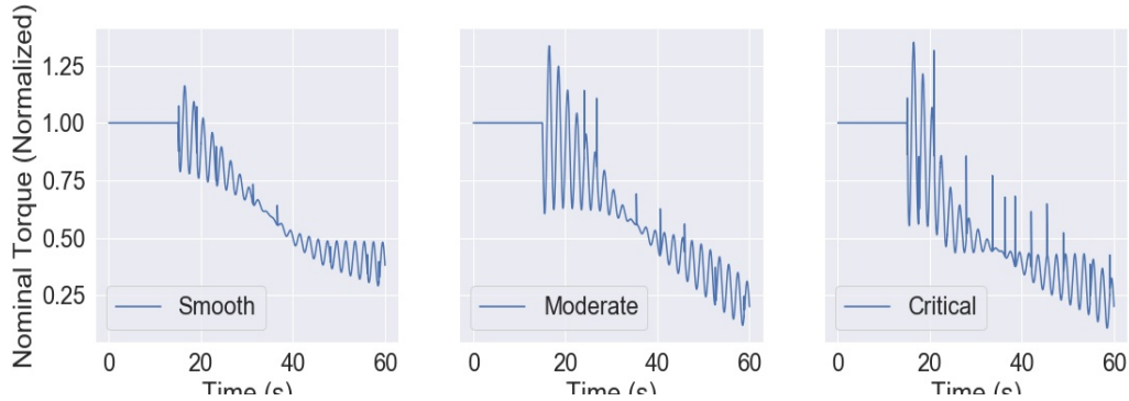
Figure 9 - Normalized nominal torque with smooth, moderate and critical non-idealities.
