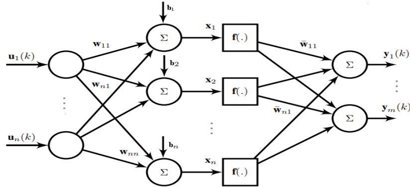
Figure 42 - Multilayer perceptron.
