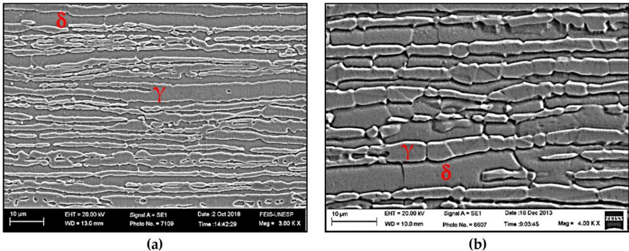
Figure 4. SEM pictures of the base material as received. (a) Reveals a balanced austenite/ferrite microstructure, with elongated geometry due to the lamination process; (b) Detail of austenite in high relief and ferrite in low relief due to Beraha etching.
