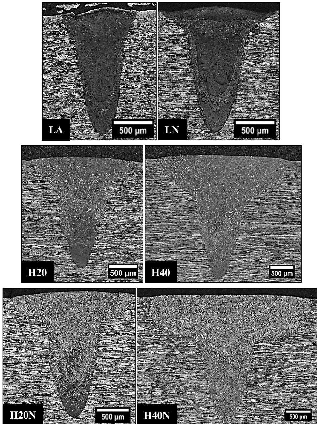
Figure 7. OM of weld bead cross sections. The %V of austenite in FZ increased from samples LA to H40N due to higher values of heat input and nitrogen addition.
