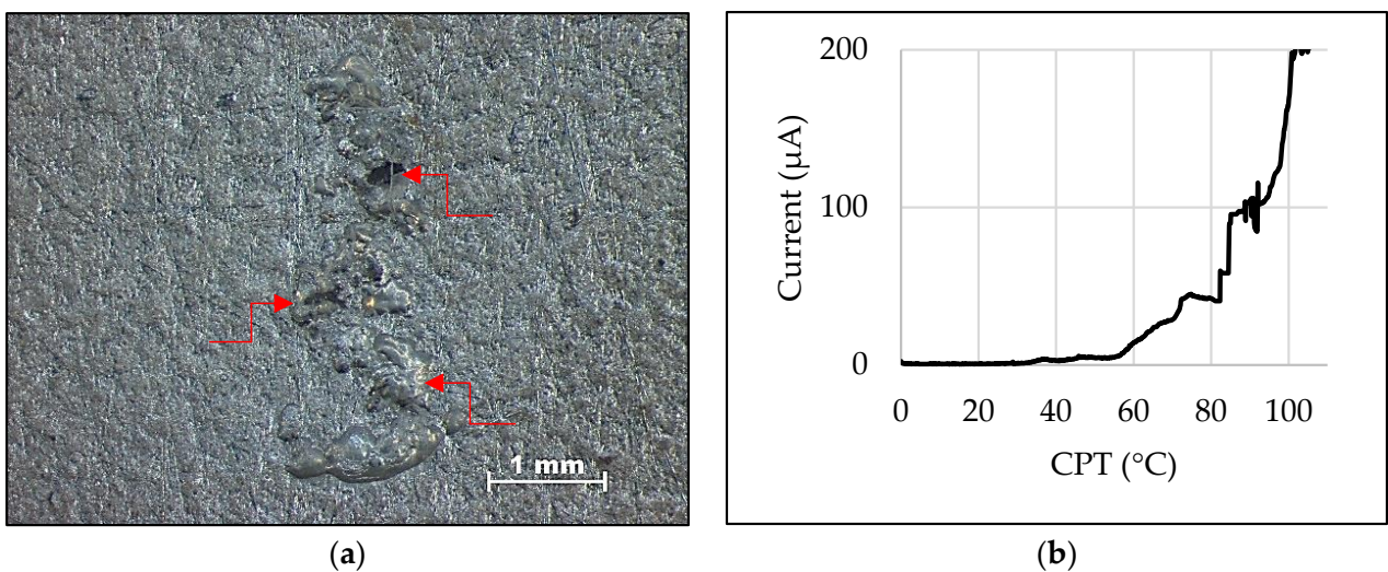
Figure 5. (a) Base metal surface after the CPT test. Arrows indicate pitting corrosion. (b) CPT test graph of the base metal, showing the current reaching 100 \mu\text{A} at a temperature of 92 °C.
