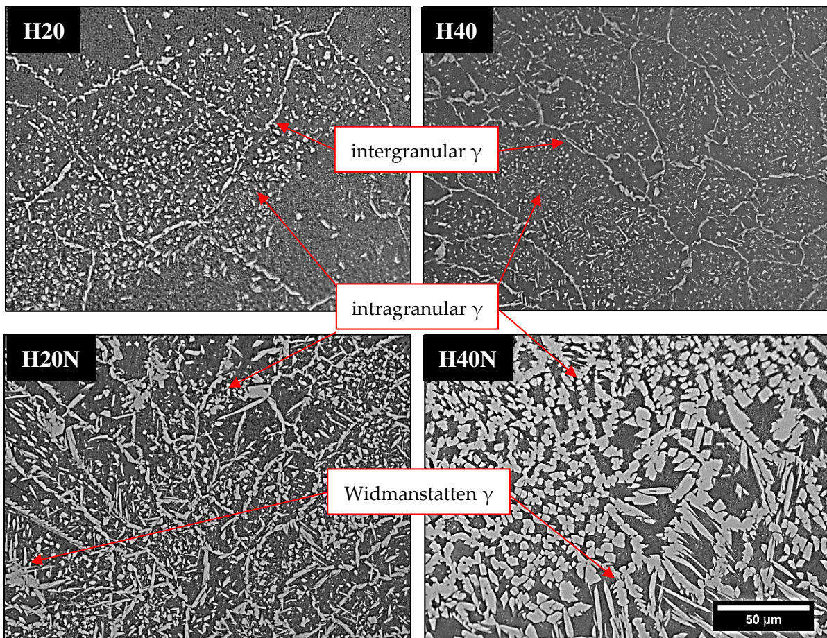
Figure 10. OM of weld bead sections H20, H40, H20N and H40N. The %V of austenite in FZ increased with higher values of heat input and nitrogen addition.
