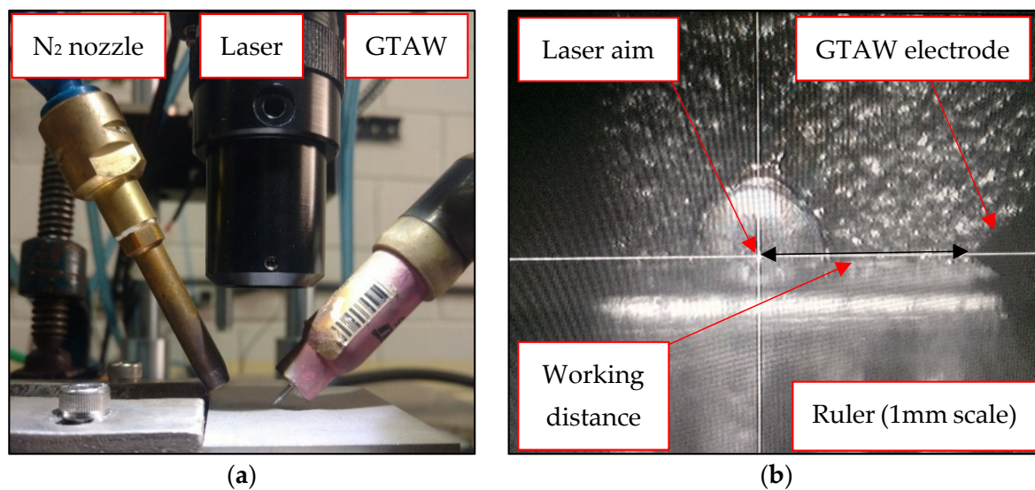
Figure 3. (a) Hybrid GTAW laser welding arrangement. (b) Laser camera view.
