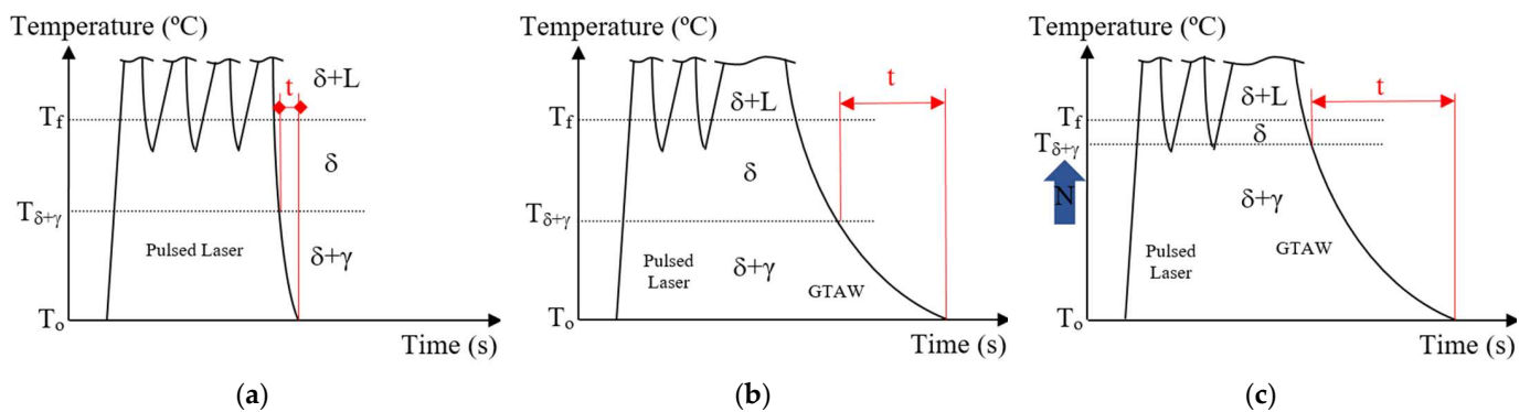
Figure 2. Time ( t ) the fusion zone remains in biphasic zone ( \delta + \gamma ) while cooling in (a) pulsed laser Nd-YAG welding, (b) hybrid GTAW pulsed laser welding and (c) hybrid GTAW pulsed laser welding with nitrogen addition.
