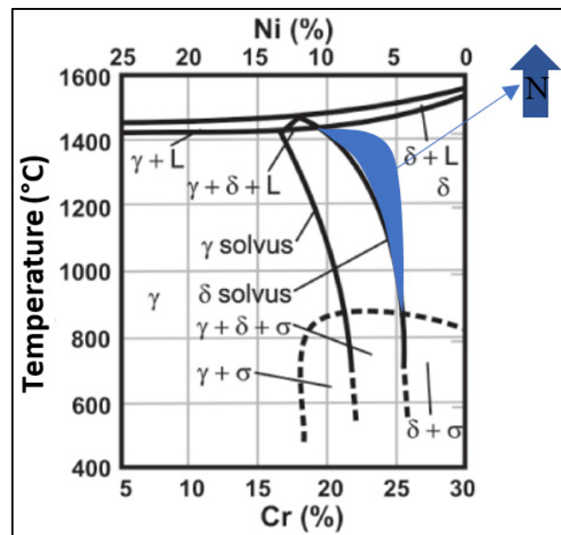
Figure 1. Cr–Ni–68%Fe pseudobinary diagram adapted by the authors [11]. The addition of N_2 expands the biphasic \delta + \gamma field.
