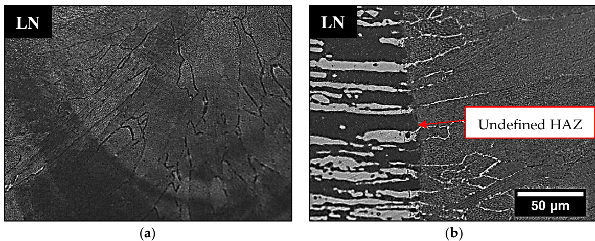
Figure 9. OM of LN weld bead where (a) the \gamma is imperceptible and (b) there is an undefined HAZ.
