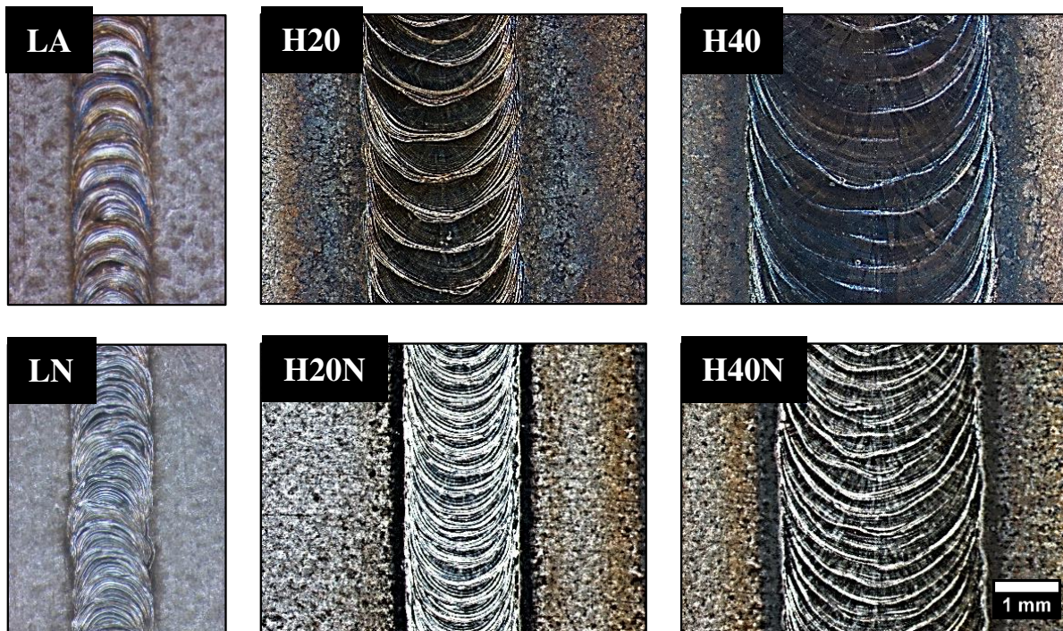
Figure 6. Top view of the weld beads. No visual defects found.
