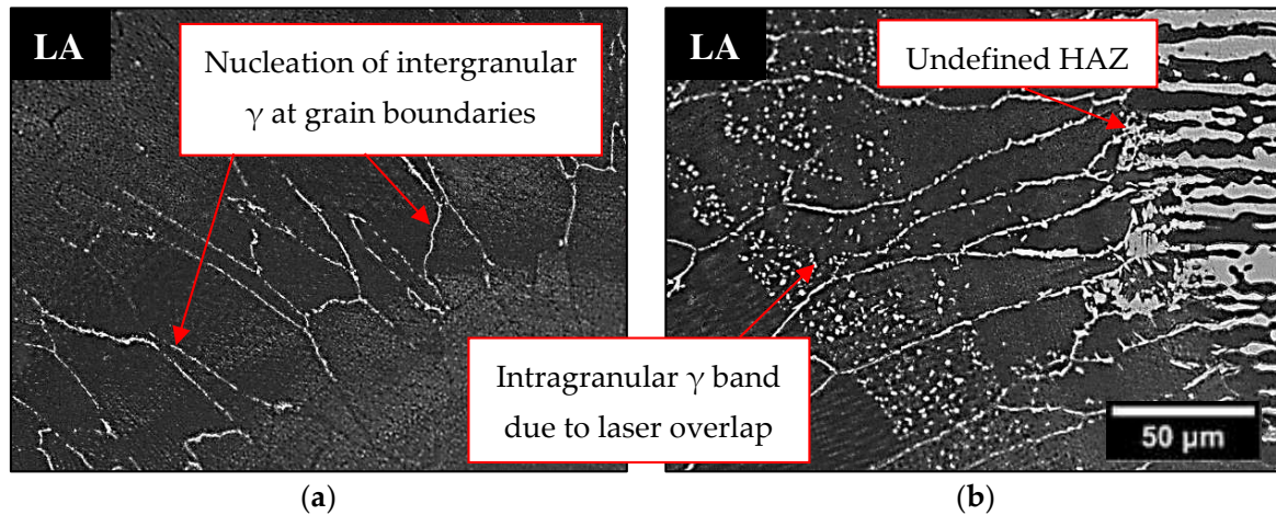
Figure 8. OM of LA weld bead showing (a) intergranular \gamma and (b) the effect of laser overlap on \gamma dispersion.
