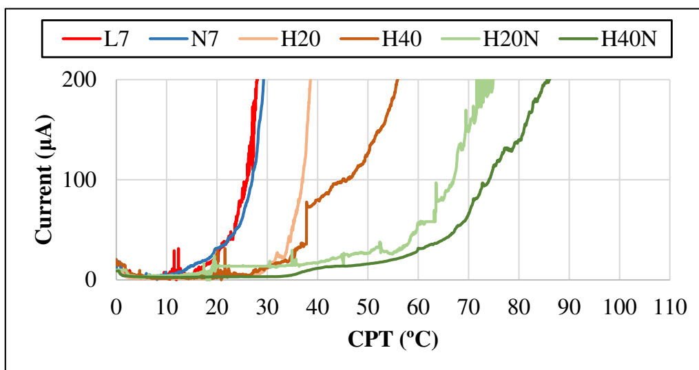
Figure 11. Graph with CPT test curves from each weld bead and base metal, showing the current reaching 100 \mu\text{A} .
