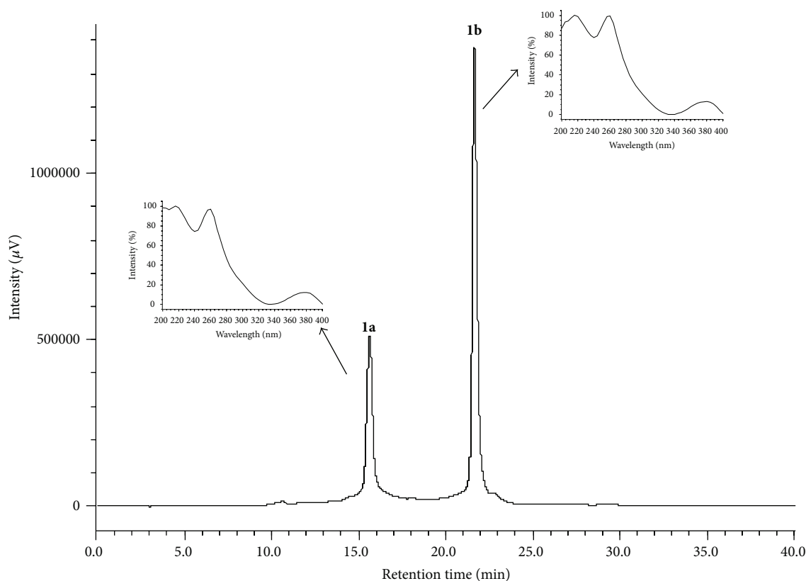
FIGURE 5: Chromatogram peak 1a ( \alpha -punicalagin) and peak 1b ( \beta -punicalagin) collected from \text{H}_2\text{O}:\text{MeOH} (8:2 v/v) at 10 mg/mL of the leaves of T. catappa , eluting at t_r 15.29 min ( 1a ) and t_r 21.07 min ( 1b ). The flow rate was 1 mL/min with a gradient 5–30% MeOH for 30 minutes using a hydro column. HPLC-PDA (Jasco), 270 nm. The UV spectra of peak 1, eluting at t_r 15.29 min ( 1a ) and at t_r 21.07 min ( 1b ), characteristic of the \alpha - and \beta -punicalagin anomers.
